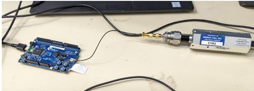
Figure 7 – Test setup – conducted antenna port measurements
