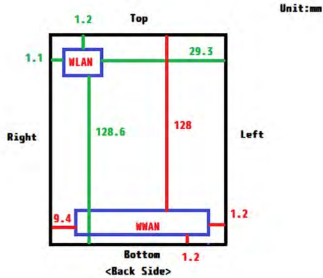
Fig.13 Antenna location
