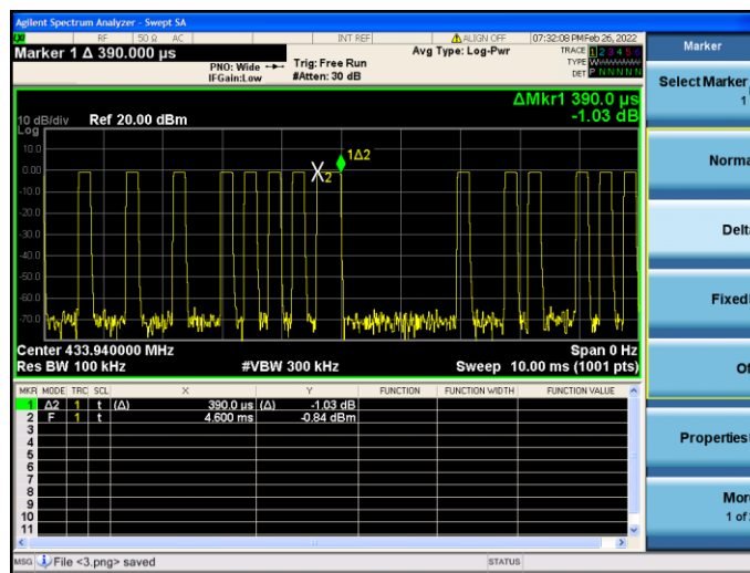
(Time per burst: 0.390ms*1pcs)
