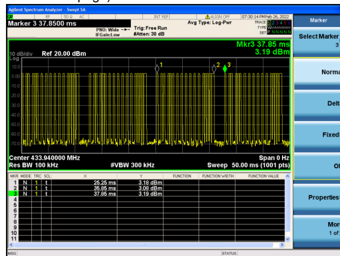
(Transmit cycle 12.60ms)
