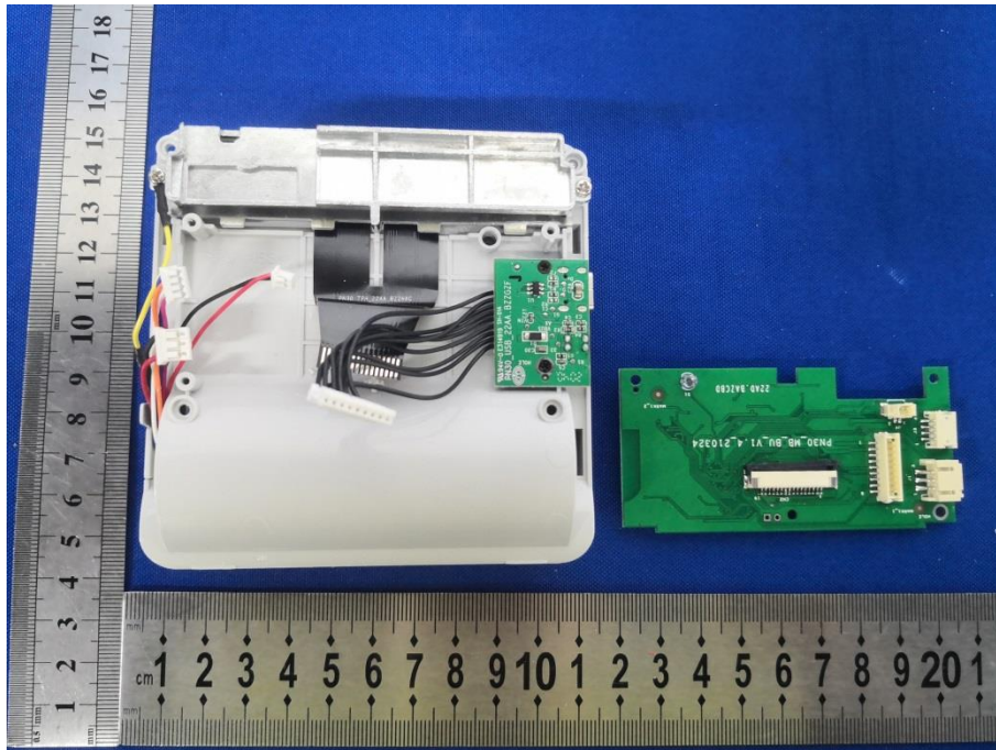
Inside View of Main Board Removed
