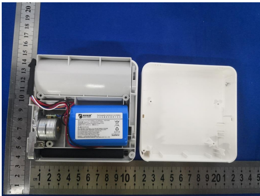
Inside view of Bottom Side
