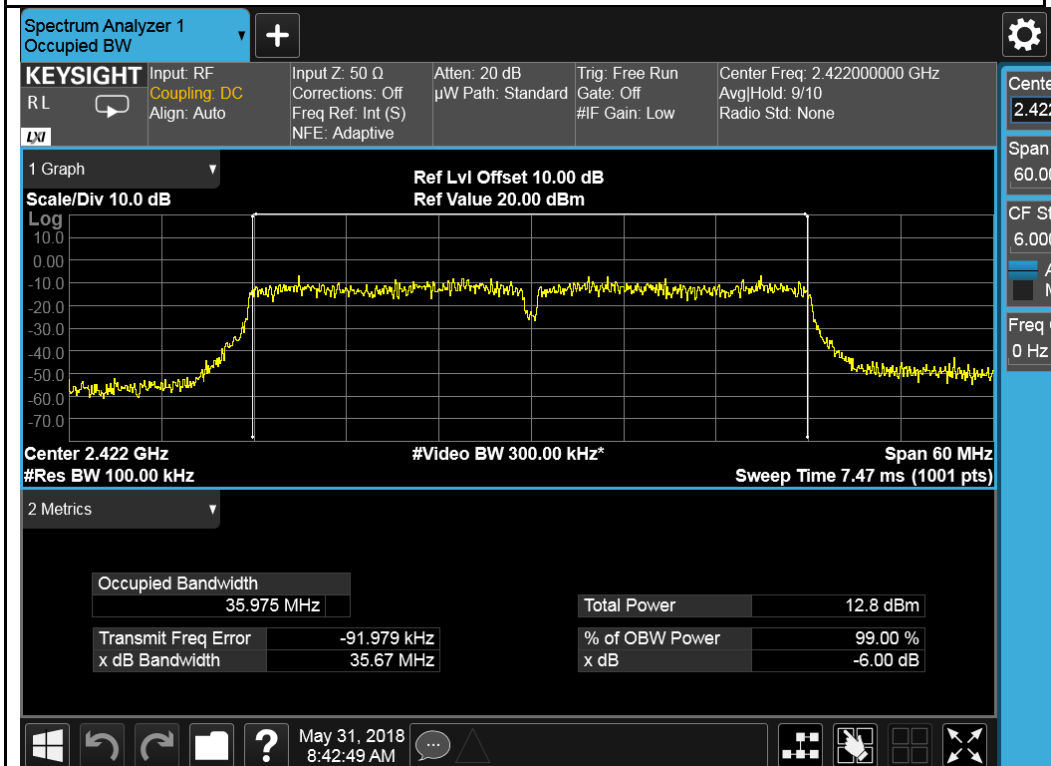
802.11n-HT40-2422MHz
