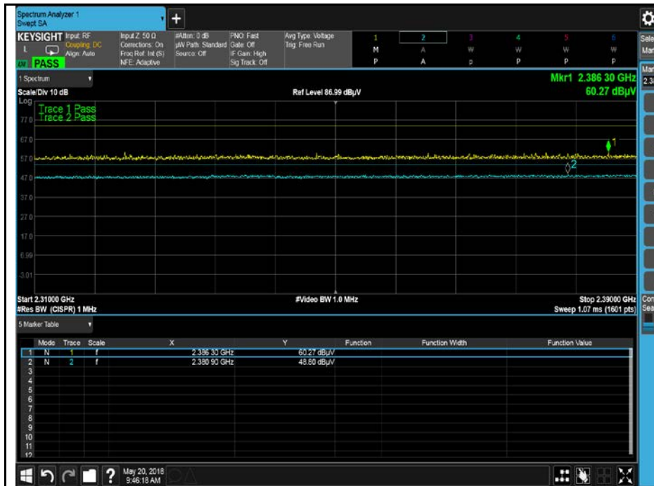
802.11n-HT40-2422MHz
