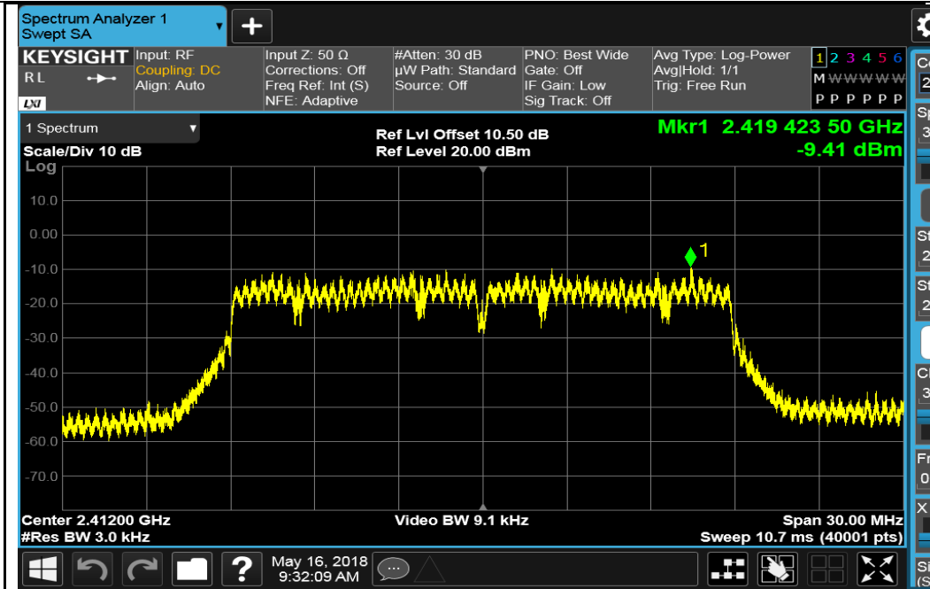
802.11n HT20- 2412MHz
