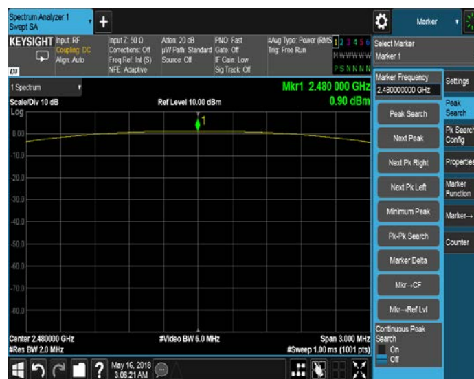
Output Power –Bluetooth LE 2480MHz
