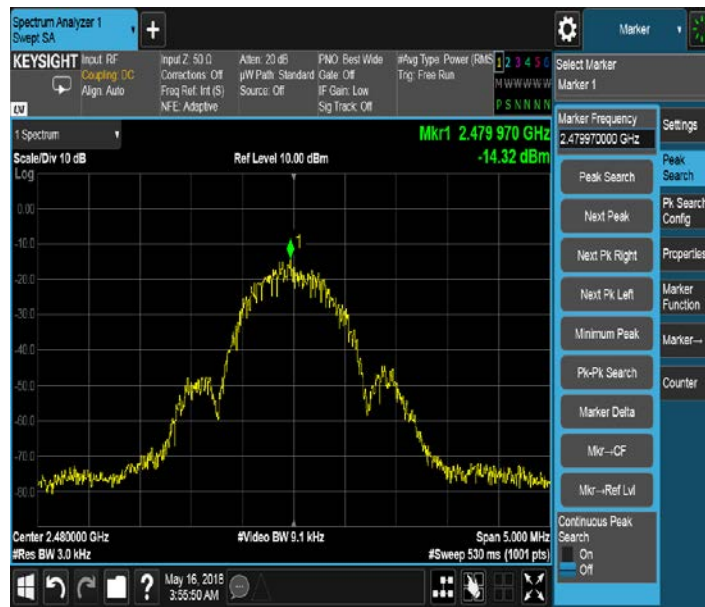
PSD -Bluetooth LE High
