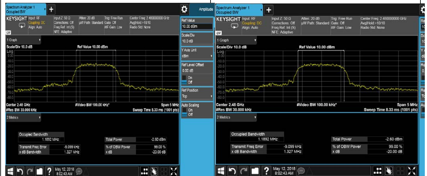
20dB BW –Bluetooth BDR 2480MHz
