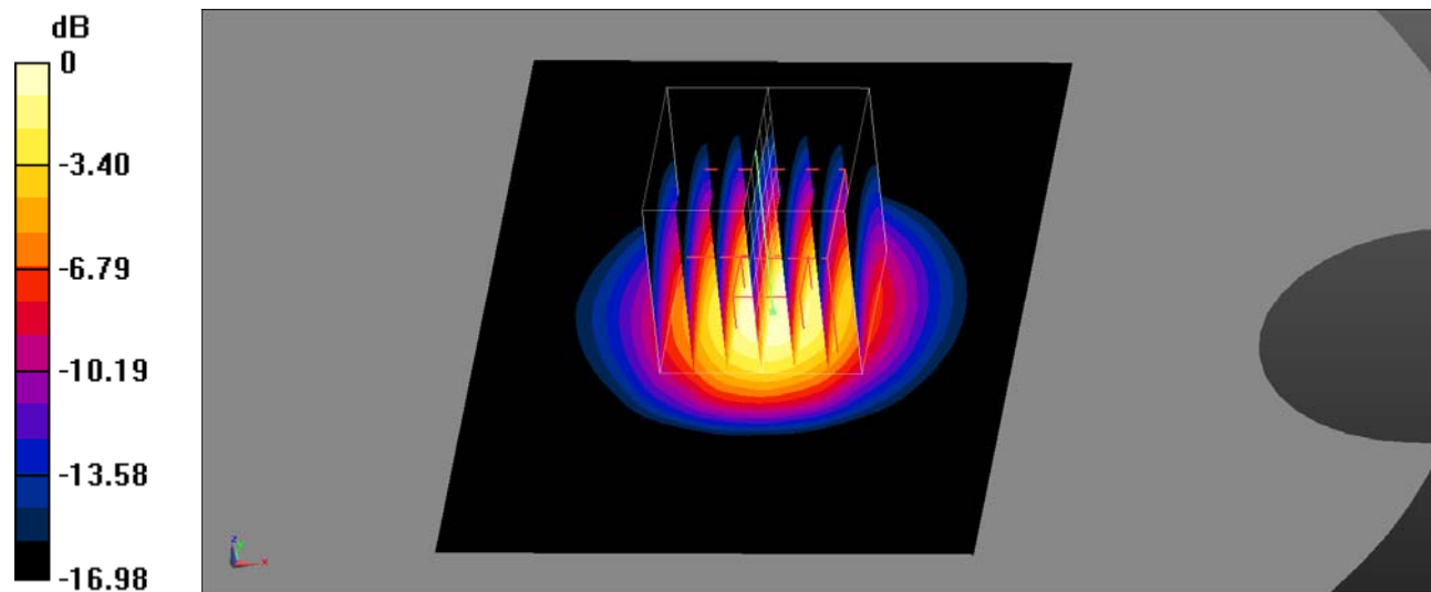
0 dB = 1.65 W/kg = 2.17 dBW/kg
