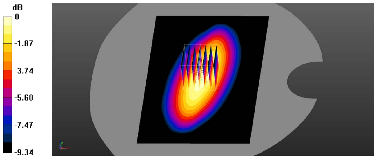
0 dB = 0.443 W/kg = -3.54 dBW/kg
