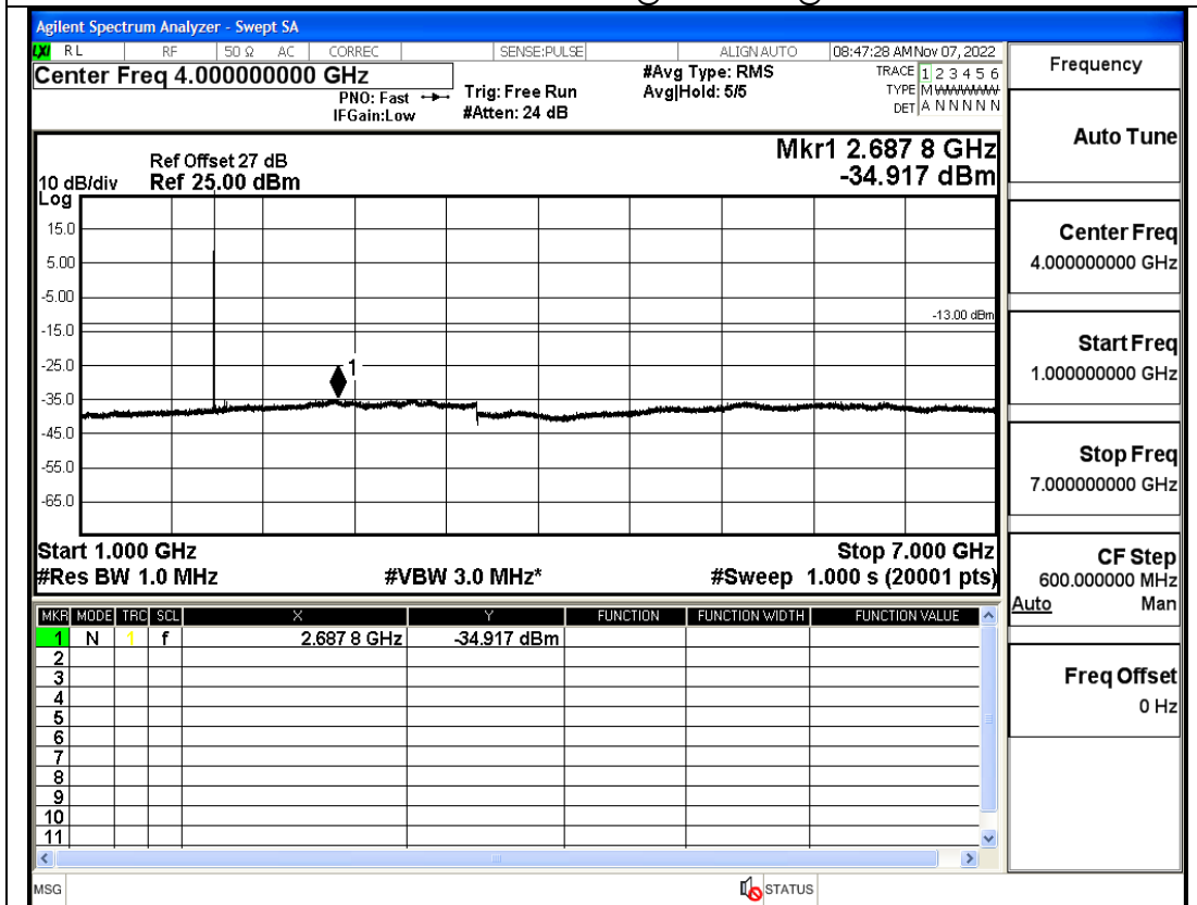
GSM1900-1880MHz-Voice@7GHz-13.6GHz@Pass
