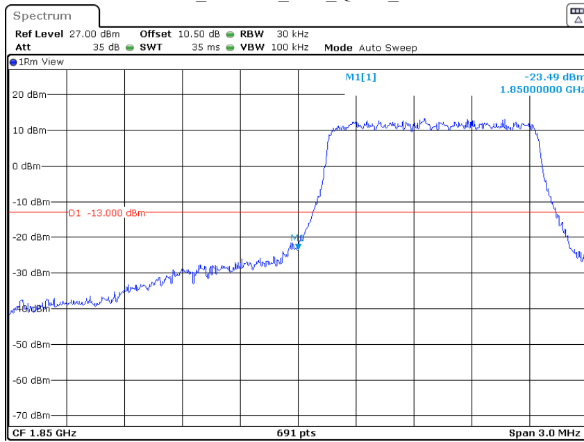
Band 2_1.4 MHz_Low_QPSK_RB6#0
