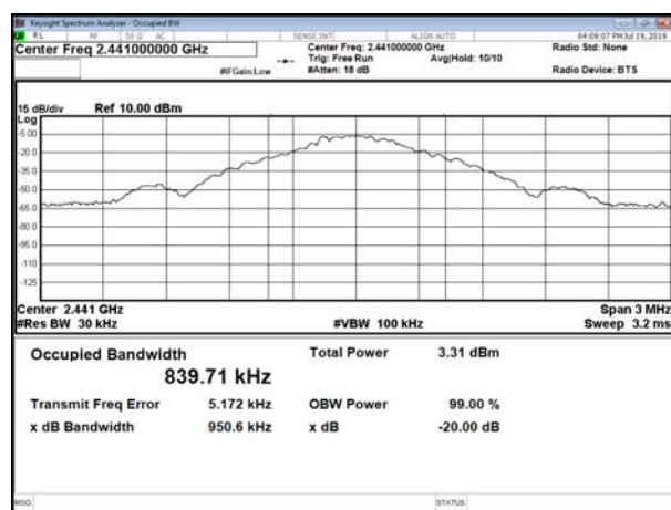
Channel 39 (2441MHz)
