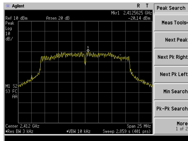
(802.11g) channel 1
