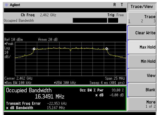
(802.11g) channel 11
