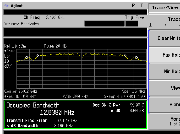
(802.11b) channel 11
