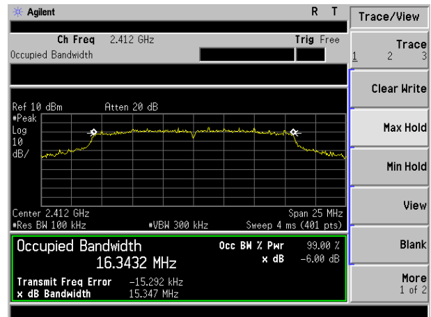
(802.11g) channel 1
