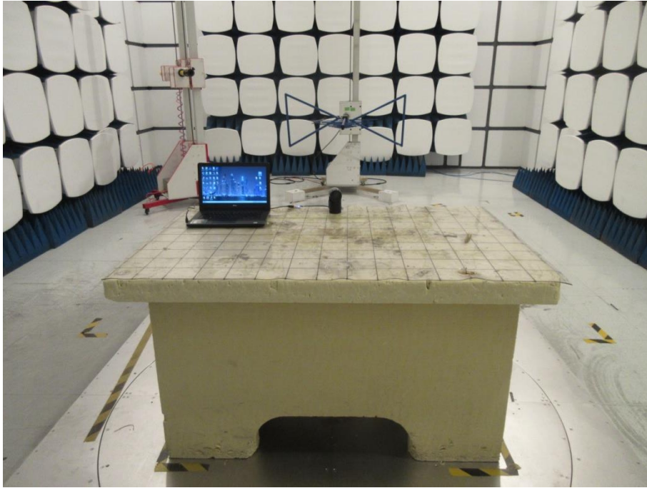
Radiated Spurious Emission Set-up photo, Up to 1GHz
