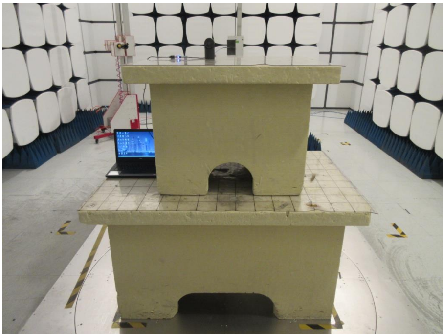
Radiated Spurious Emission Set-up photo, Above 1GHz
