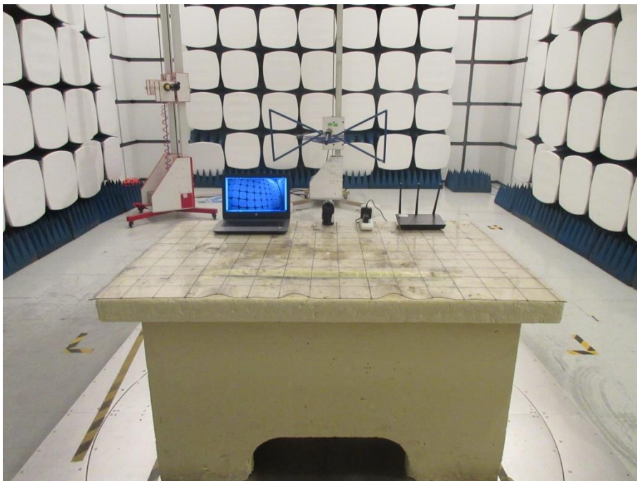
Radiated Emission Set-up Photo, Up to 1GHz
