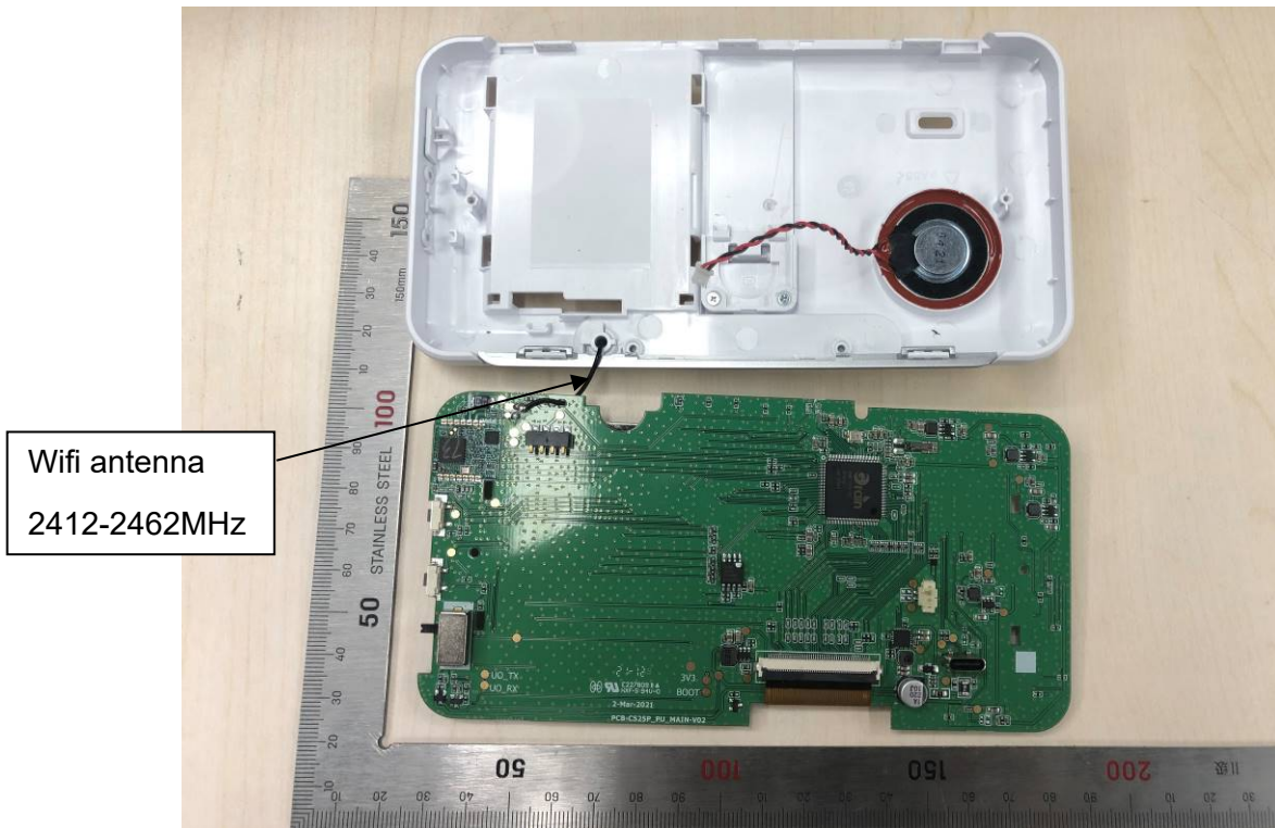
Fig. 2. Parent unit internal view -3
