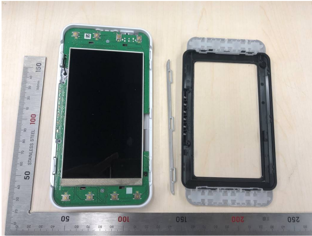
Fig. 1. Parent unit internal view -2
