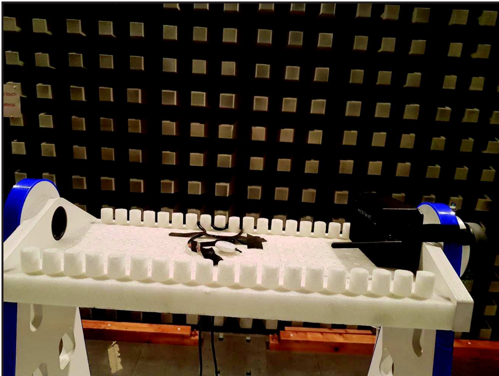
Photo 4: The Black Box is Arendi Bluetooth Tester (ABT) placed at closer distance to EUT so that it transmits maximum power levels.
