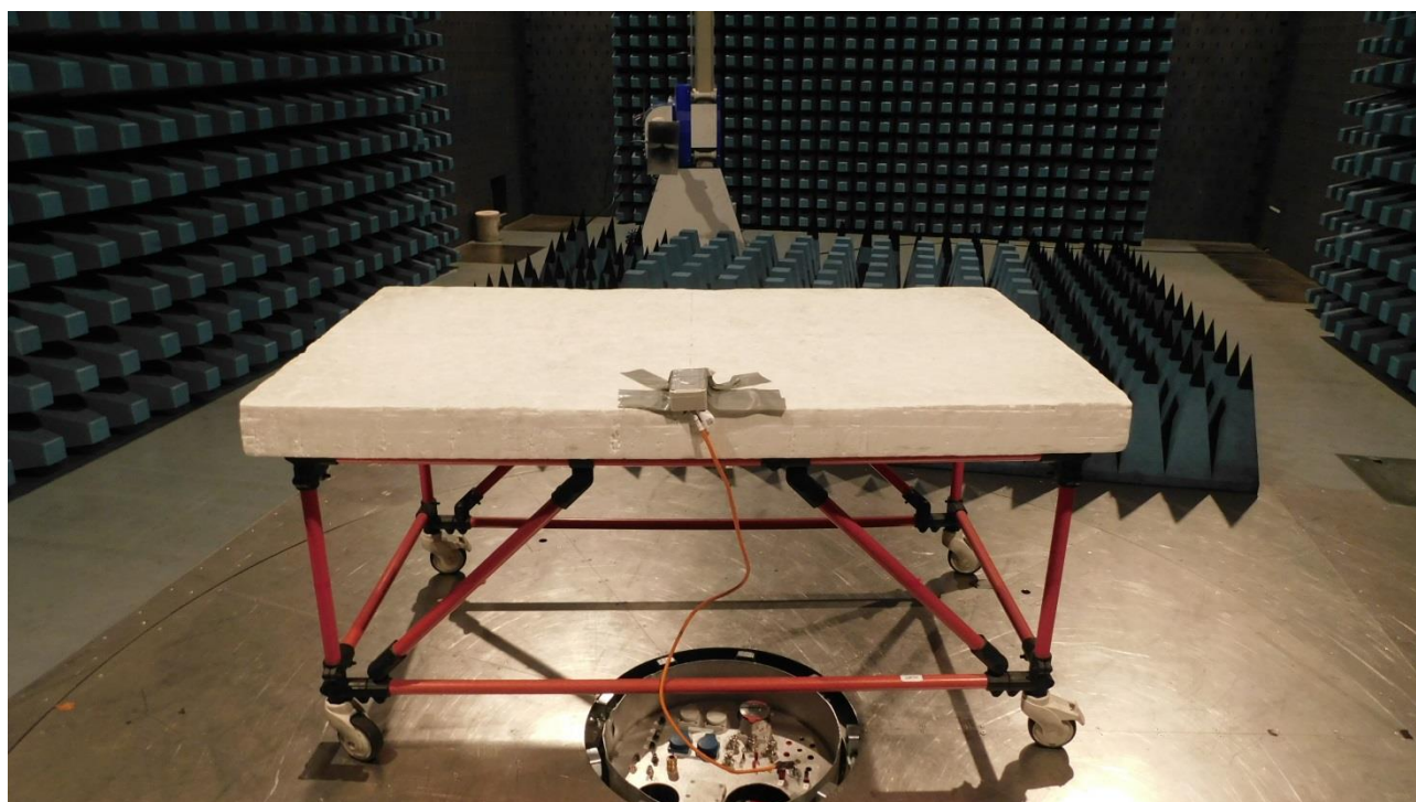
Picture 3: EUT test setup radiated emission test > 1 GHz (front view)
