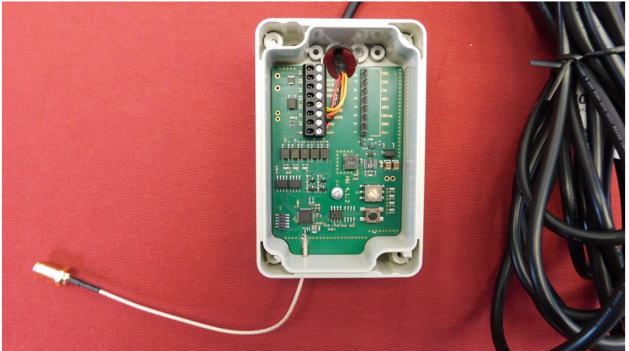
Picture 1: Opened EUT with antenna cable - top side
