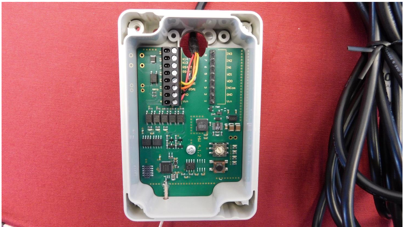
Picture 3: Opened EUT with original antenna – top side
