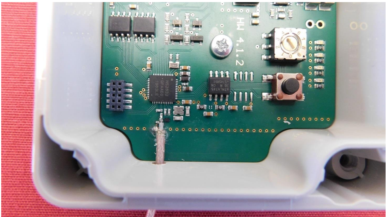
Picture 2: Opened EUT with antenna cable – detailed view
