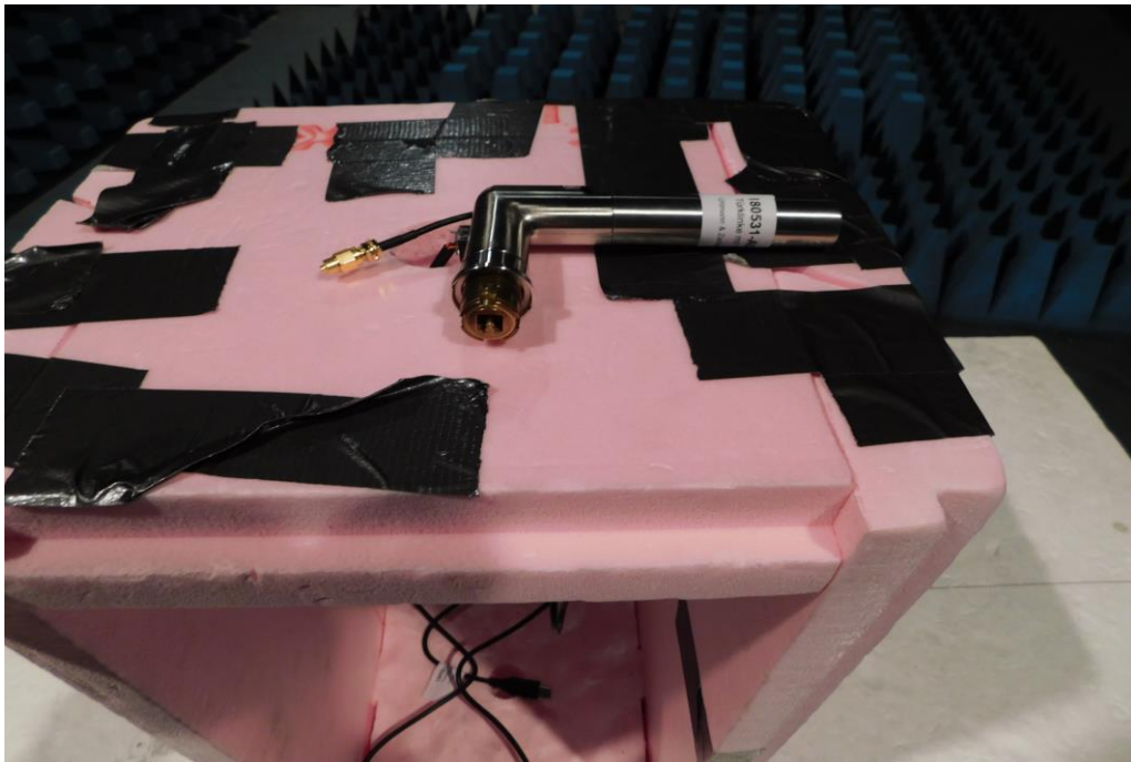
Picture 1: EUT position 1 – top view
