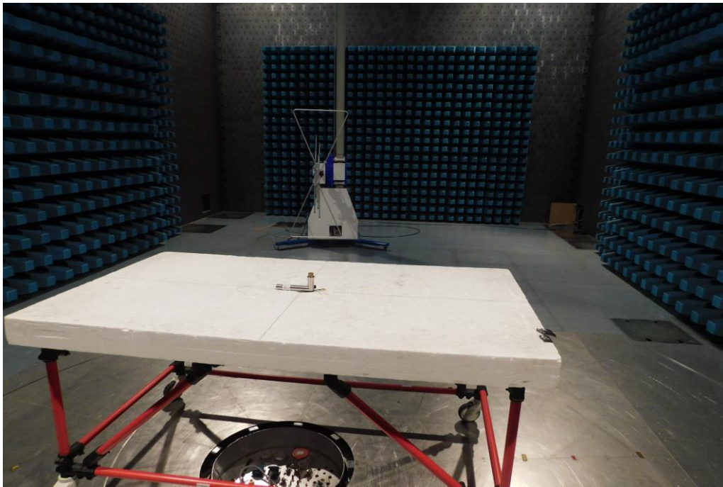
Picture 5: SAC, radiated emission test 30 MHz – 1 GHz – position 2 (front view)
