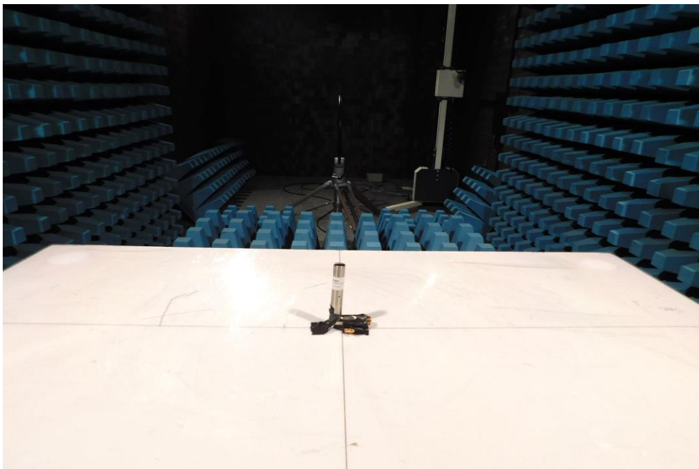
Picture 4: CDC, radiated emission test 9 kHz -30 MHz – position 3 (front view)
