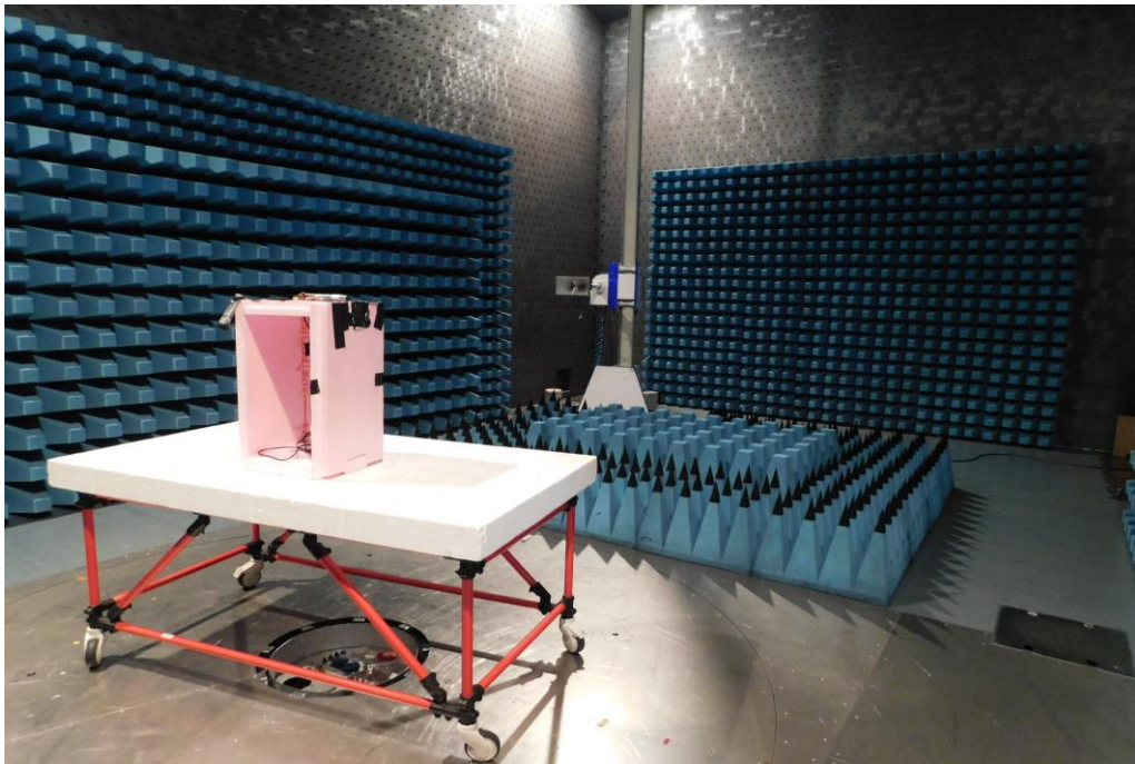
Picture 7: SAC, radiated emission test 1 GHz – 16 GHz – position 1 (front view)
