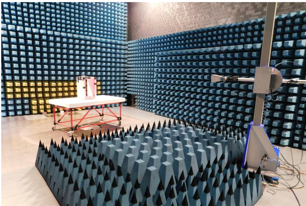
Picture 8: SAC, radiated emission test 1 GHz – 16 GHz – position 1 (front view)
