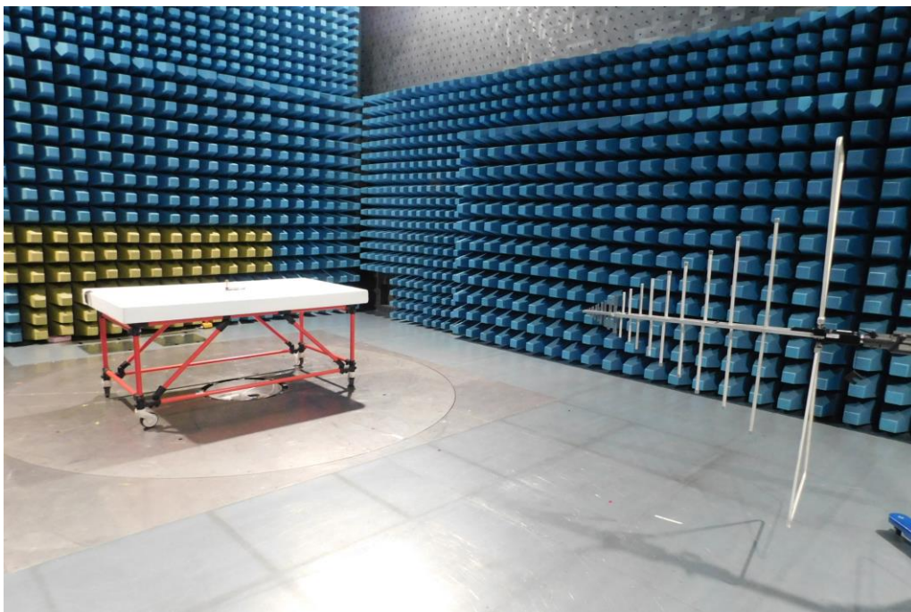
Picture 6: SAC, radiated emission test 30 MHz – 1 GHz – position 2 (rear view)
