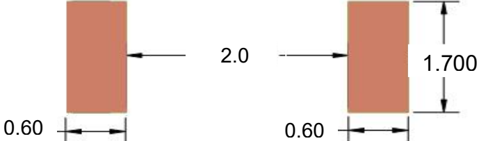
FootPrint (Unit : mm)
