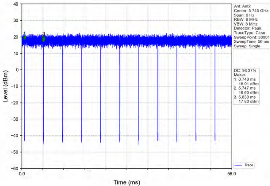
802.11n(HT20)_LCH_5745MHz_Ant2_NTNV
