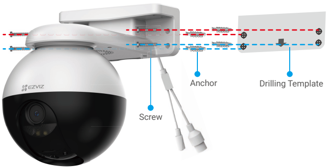
Fig. 2 Wall Mount
