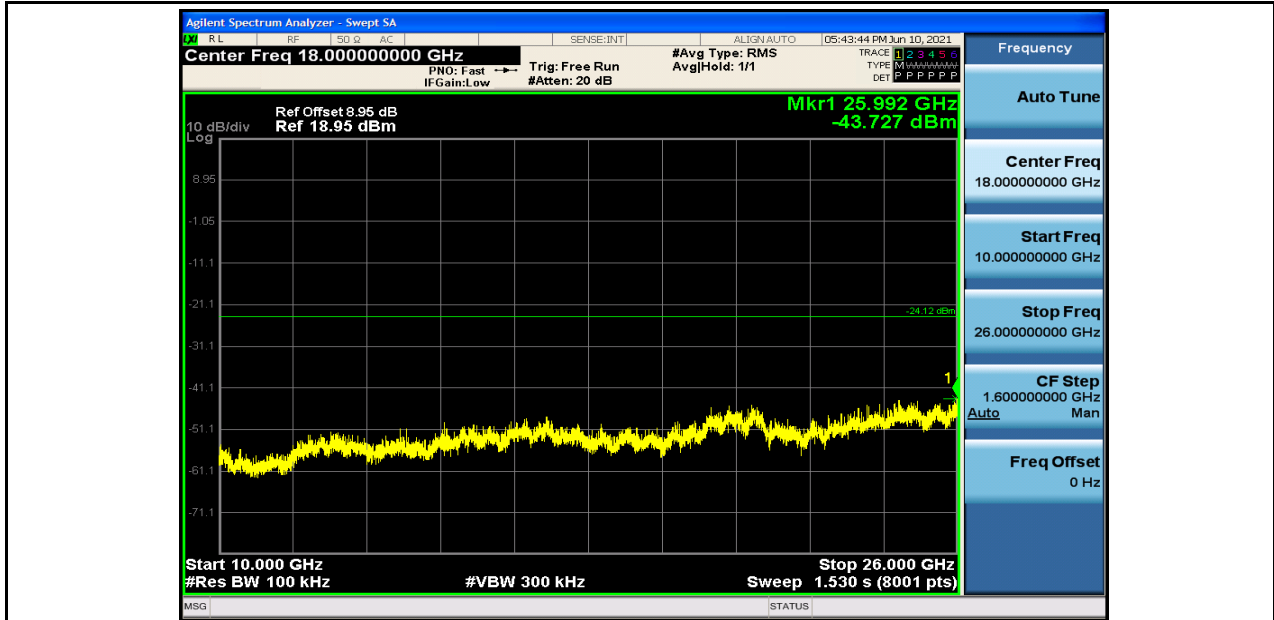
RF Conducted Spurious Emissions_11G_2412_Ant1
