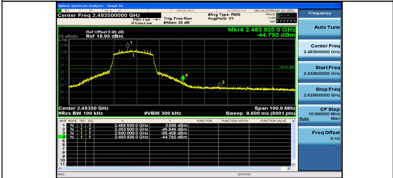
Band-edge for RF Conducted Emissions_11N20MIMO_2462_Ant1
