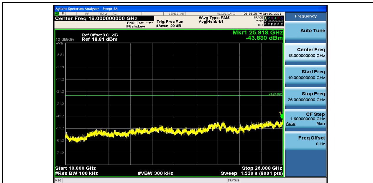
RF Conducted Spurious Emissions_11B_2437_Ant1
