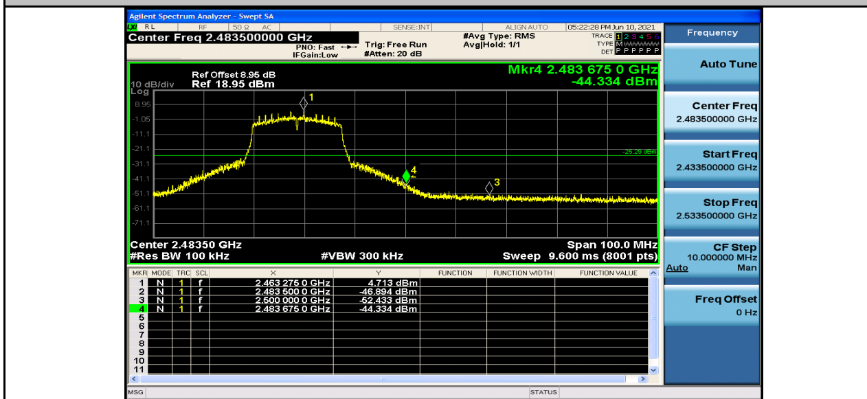
Band-edge for RF Conducted Emissions_11N20MIMO_2462_Ant2
