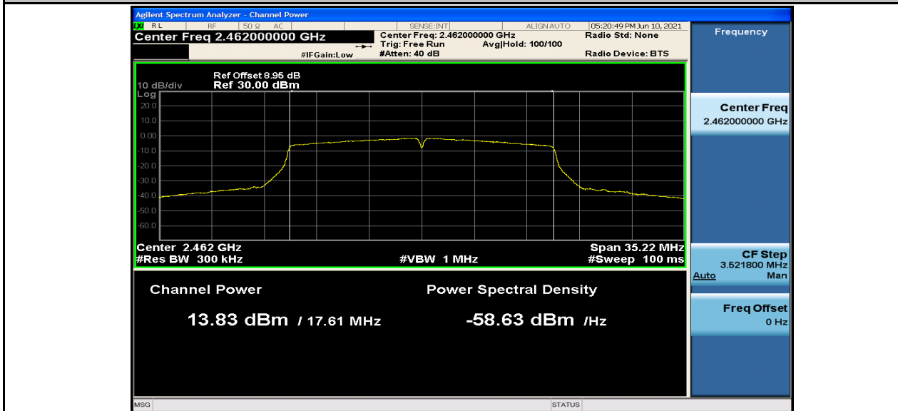
Maximum conducted (average) output power_11N20MIMO_2462_Ant2
