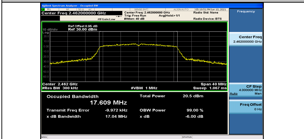
Occupied Bandwidth_11N20MIMO_2462_Ant2
