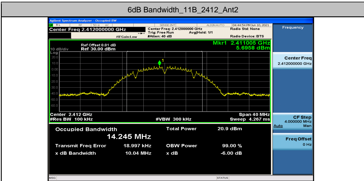
6dB Bandwidth_11B_2437_Ant2
