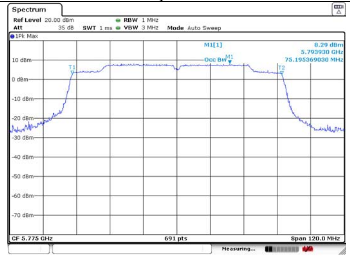
99% Occupied Bandwidth
