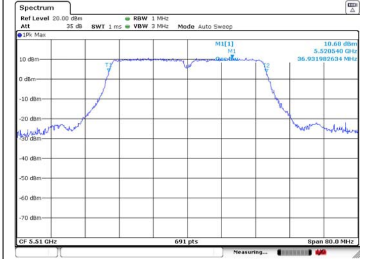
99% Occupied Bandwidth
