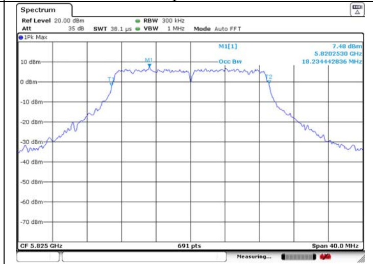
99% Occupied Bandwidth
