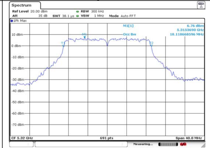
99% Occupied Bandwidth
