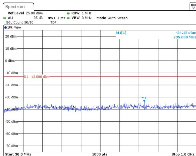
Band66-10MHz-QPSK-132022-1RB#0-Range2:1000~10000MHz
