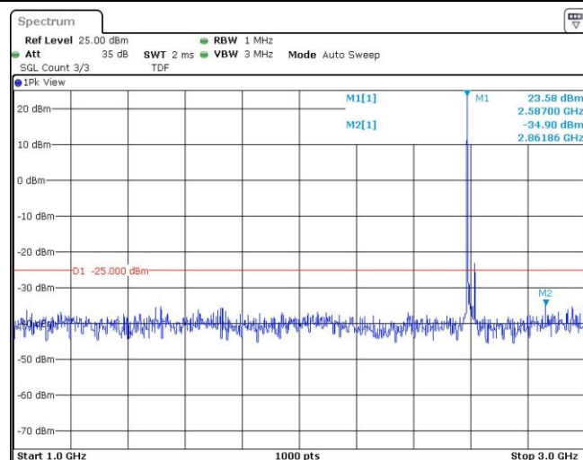
Band41-15MHz-16QAM-40620-1RB#0-Range2:1000~3000MHz
