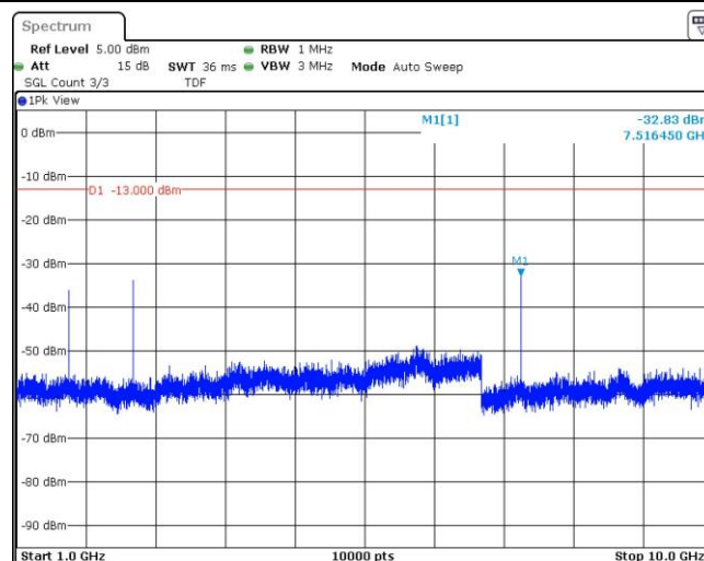
Band26-3MHz-16QAM-26915-1RB#0-Range2:1000~10000MHz
