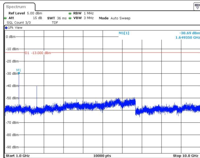
Band26-10MHz-16QAM-26915-1RB#0-Range1:30~1000MHz
