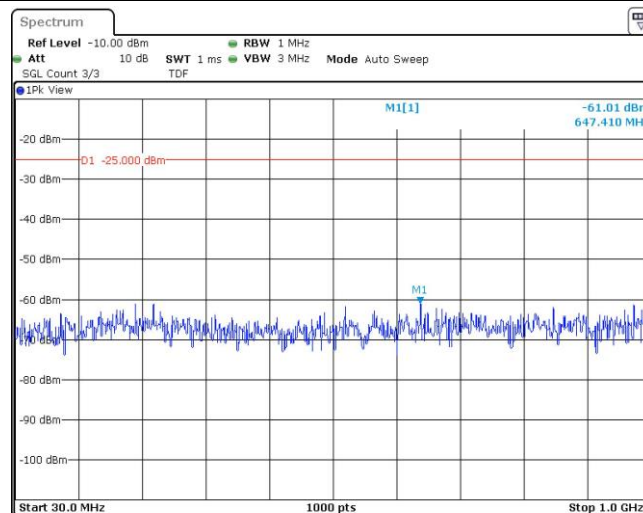
Band41-10MHz-QPSK-40620-1RB#0-Range2:1000~3000MHz
