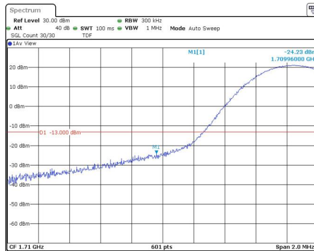
Band66-15MHz-QPSK-132047-1RB#74
