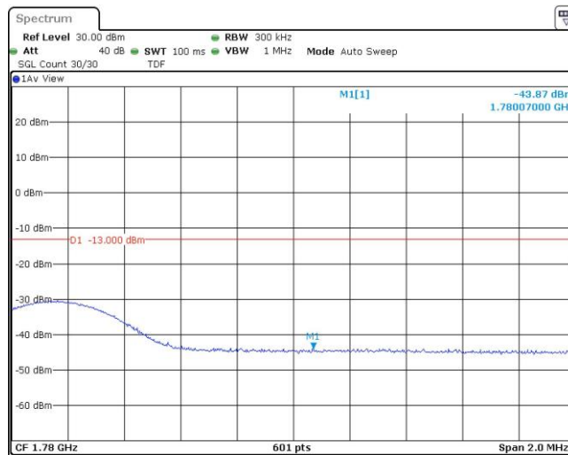
Band66-15MHz-QPSK-132597-1RB#74
