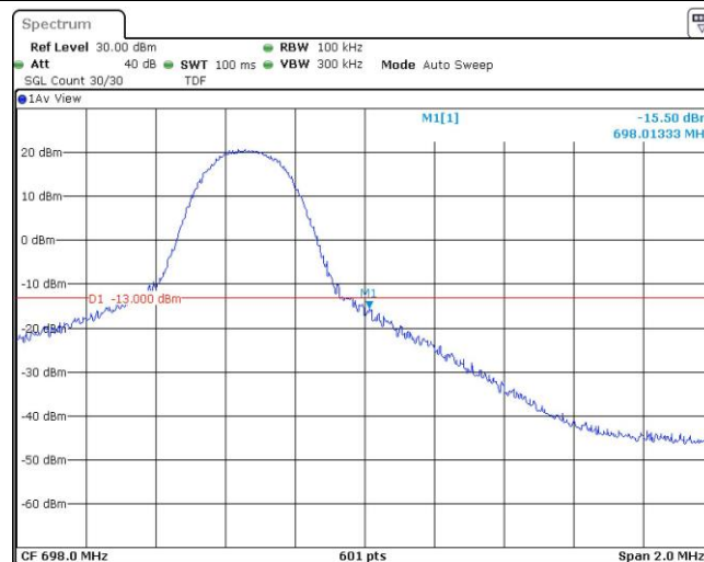
Band71-5MHz-16QAM-133447-25RB#0
