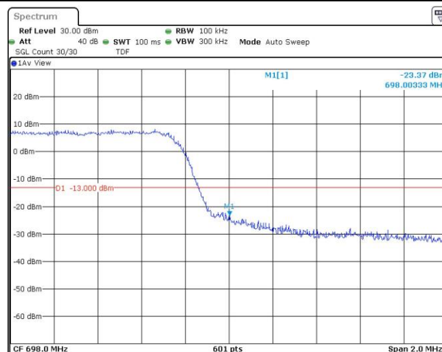
Band71-5MHz-16QAM-133147-1RB#0
