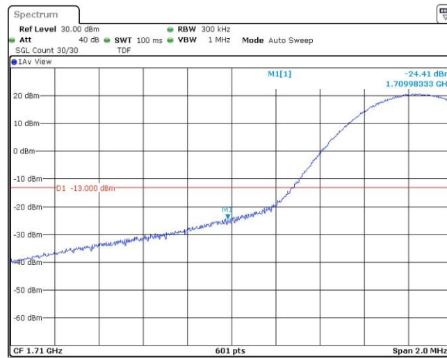
Band66-15MHz-16QAM-132047-1RB#74
