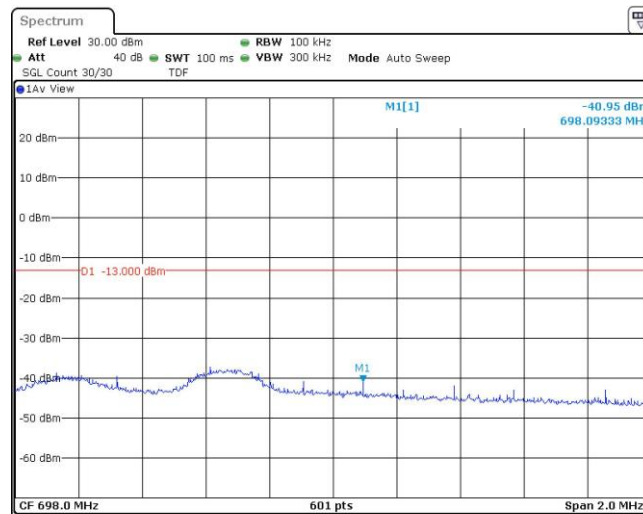
Band71-5MHz-16QAM-133447-1RB#24
