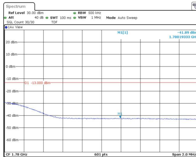
Band66-20MHz-16QAM-132572-1RB#99
