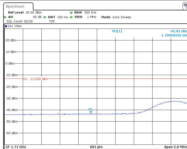
Band66-15MHz-16QAM-132047-75RB#0
