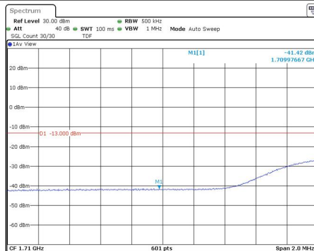
Band66-20MHz-16QAM-132072-100RB#0
