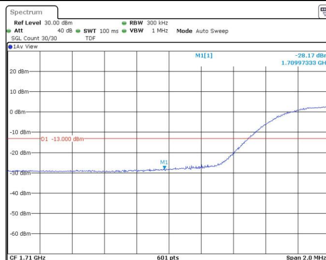
Band66-15MHz-16QAM-132597-1RB#0
