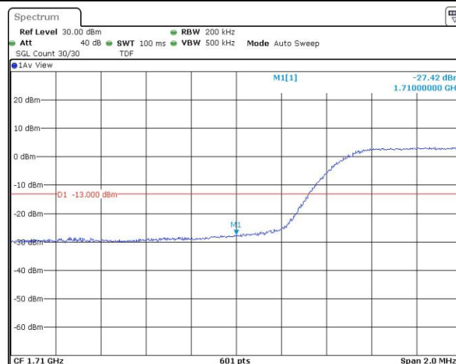
Band66-10MHz-16QAM-132622-1RB#0
