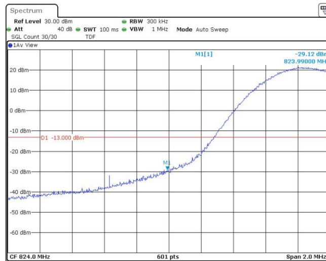
Band26-15MHz-16QAM-26865-1RB#74
