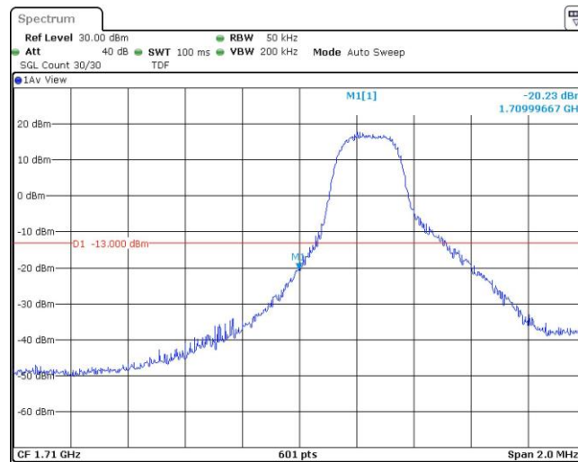
Band66-3MHz-16QAM-131987-1RB#14
