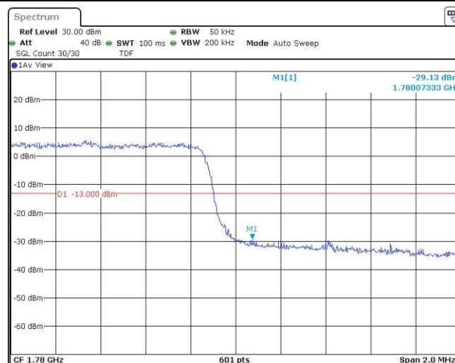
Band66-3MHz-16QAM-131987-1RB#0
