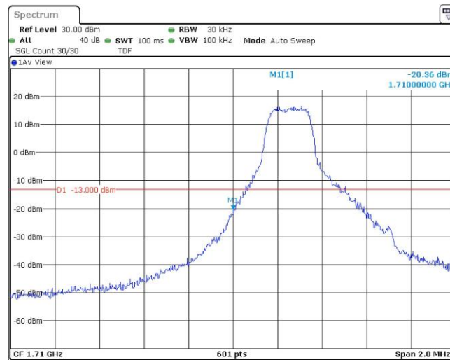
Band66-1.4MHz-QPSK-131979-1RB#5
