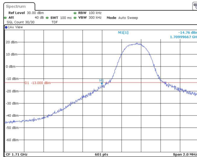
Band66-5MHz-16QAM-131997-1RB#24
