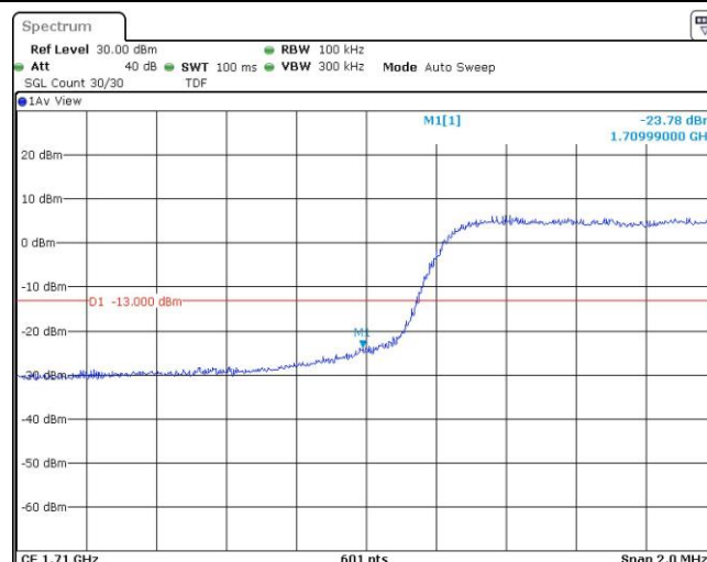
Band66-5MHz-QPSK-132647-1RB#0
