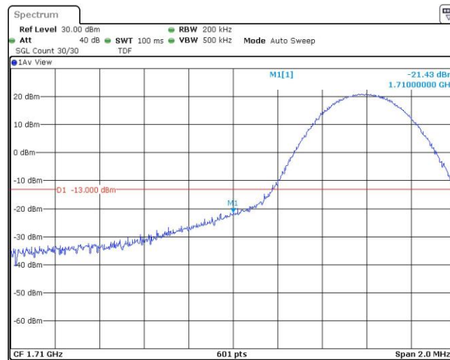
Band66-10MHz-QPSK-132022-1RB#49
