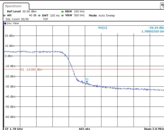
Band66-5MHz-16QAM-131997-1RB#0
