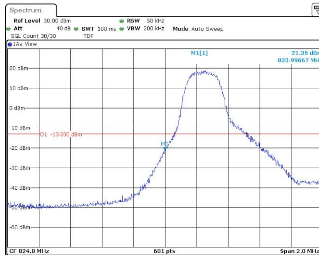
Band26-3MHz-QPSK-26805-1RB#14
