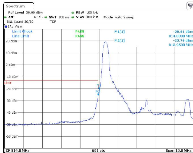
Band26-5MHz-QPSK-26715-1RB#24
