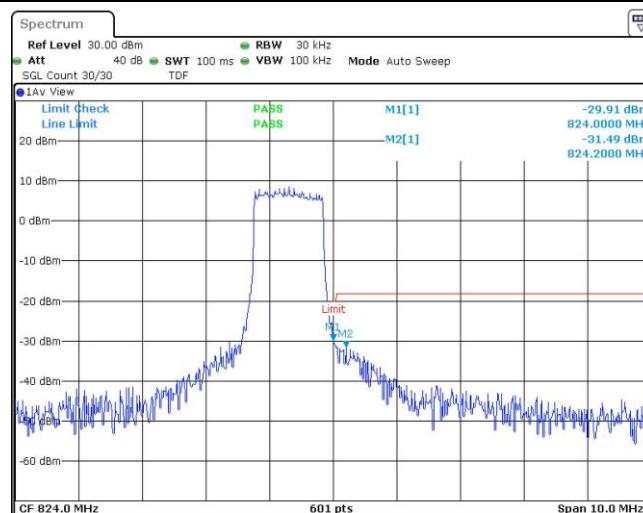
Band26-1.4MHz-16QAM-26797-1RB#0
