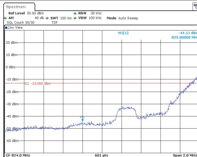
Band26-1.4MHz-QPSK-26797-6RB#0
