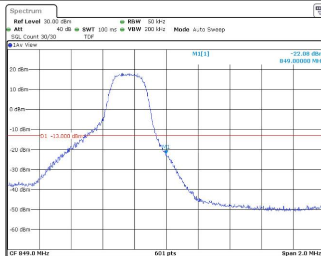
Band26-3MHz-QPSK-27025-15RB#0
