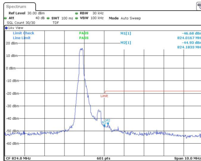
Band26-1.4MHz-16QAM-26783-1RB#5
