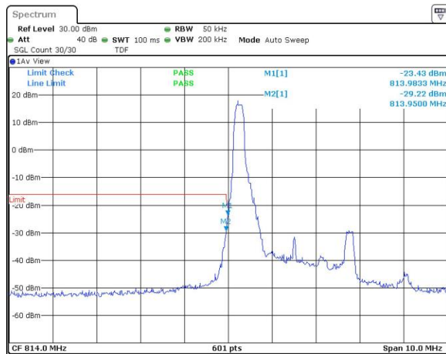
Band26-3MHz-16QAM-26705-1RB#14
