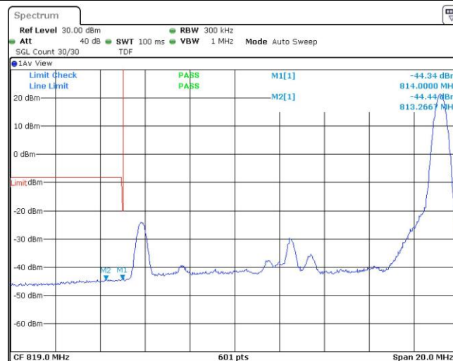
Band26-15MHz-QPSK-26765-75RB#0
