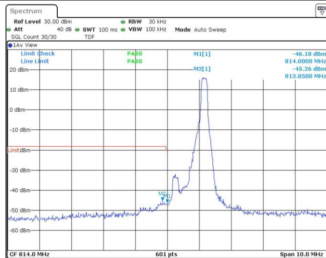
Band26-1.4MHz-QPSK-26697-6RB#0
