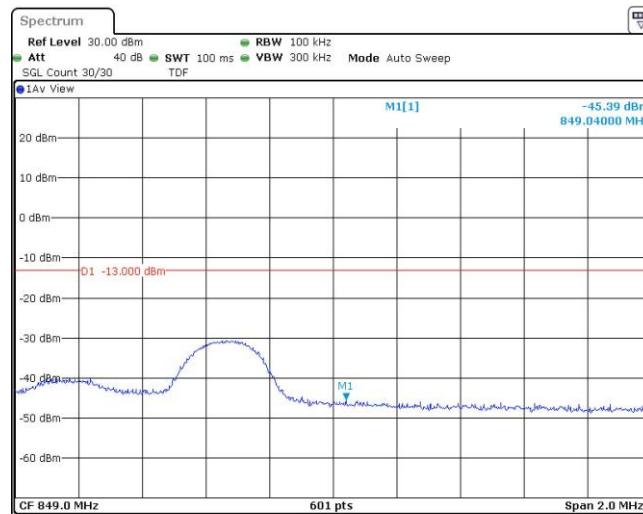
Band26-5MHz-QPSK-27015-1RB#24
