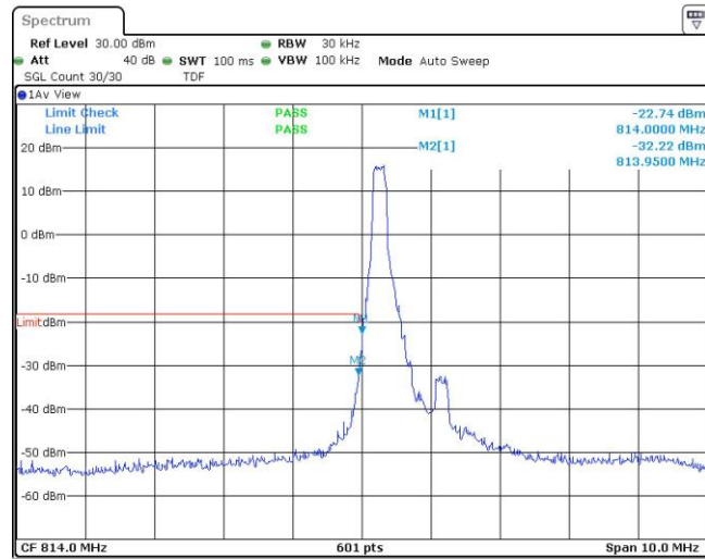
Band26-1.4MHz-16QAM-26697-1RB#5
