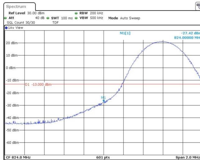
Band26-10MHz-QPSK-26840-1RB#49
