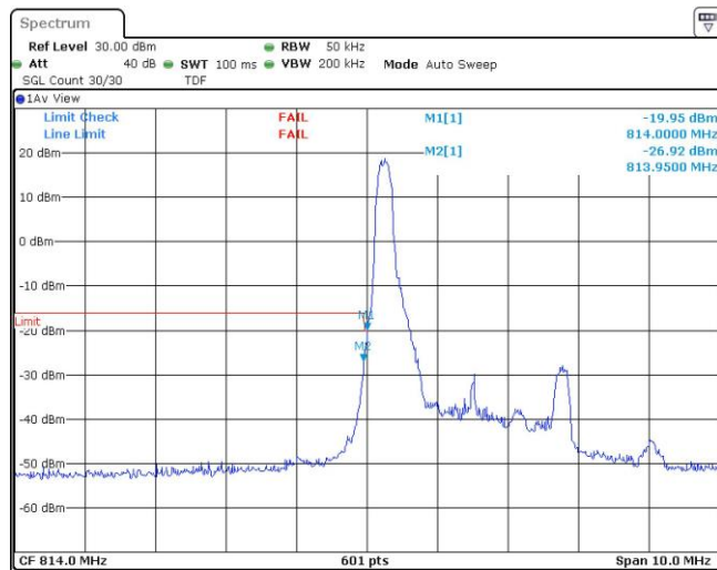
Band26-3MHz-QPSK-26705-1RB#14
