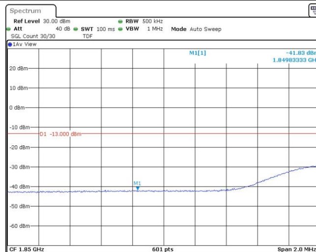
Band25-20MHz-QPSK-26140-100RB#0
