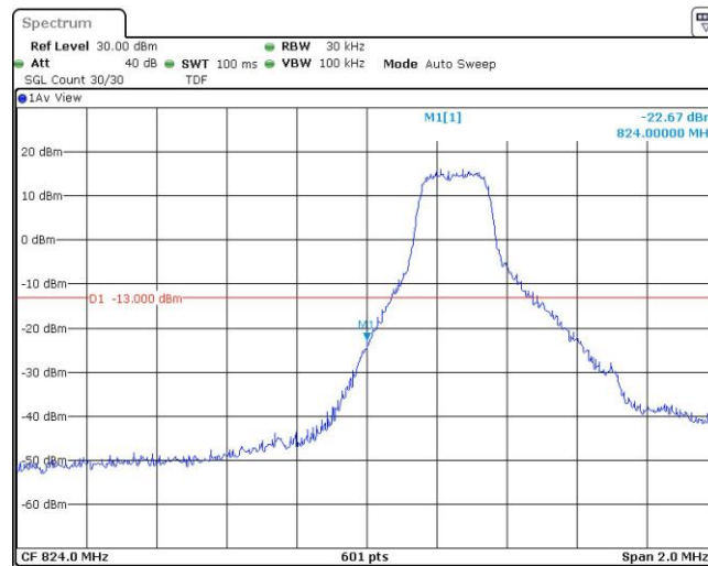
Band26-1.4MHz-16QAM-26797-1RB#5
