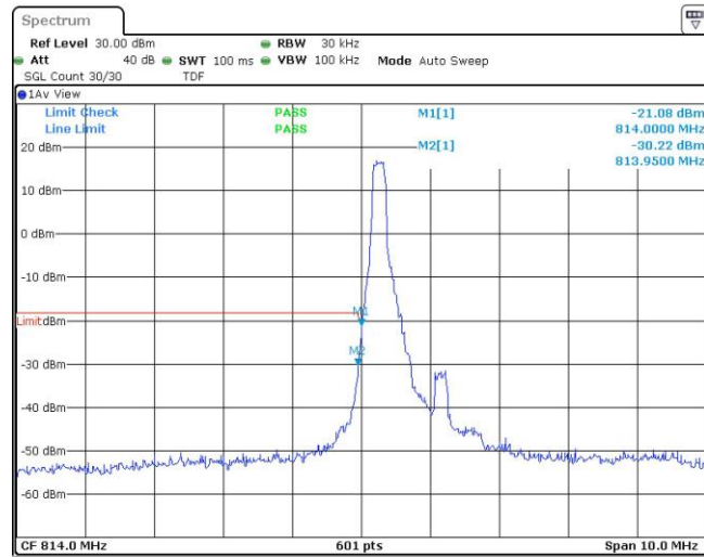
Band26-1.4MHz-QPSK-26697-1RB#5
