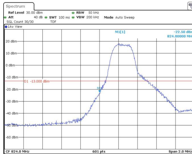
Band26-3MHz-16QAM-26805-1RB#14
