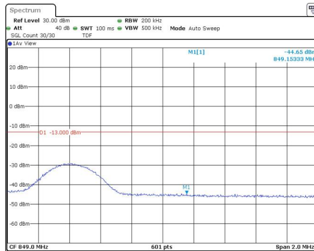
Band26-10MHz-16QAM-26990-1RB#49
