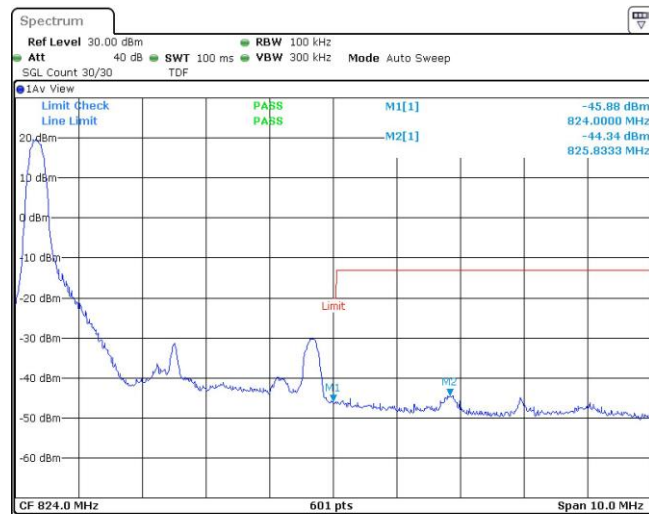
Band26-5MHz-QPSK-26765-1RB#24
