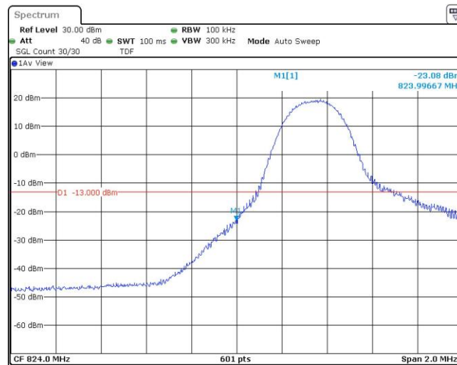
Band26-5MHz-16QAM-26815-1RB#24
