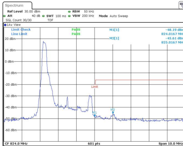
Band26-3MHz-16QAM-26775-1RB#14
