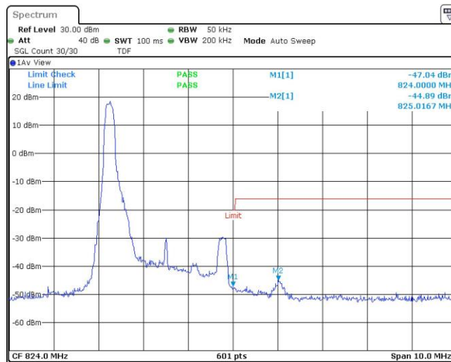
Band26-3MHz-QPSK-26775-1RB#14
