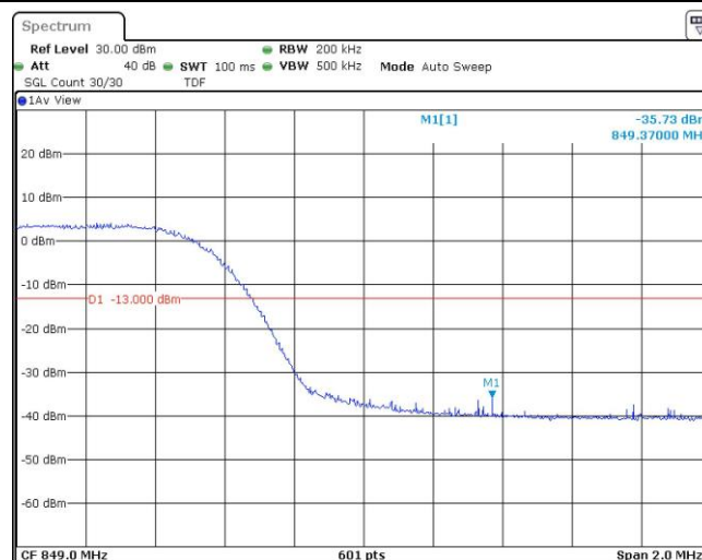
Band26-15MHz-QPSK-26765-1RB#0
