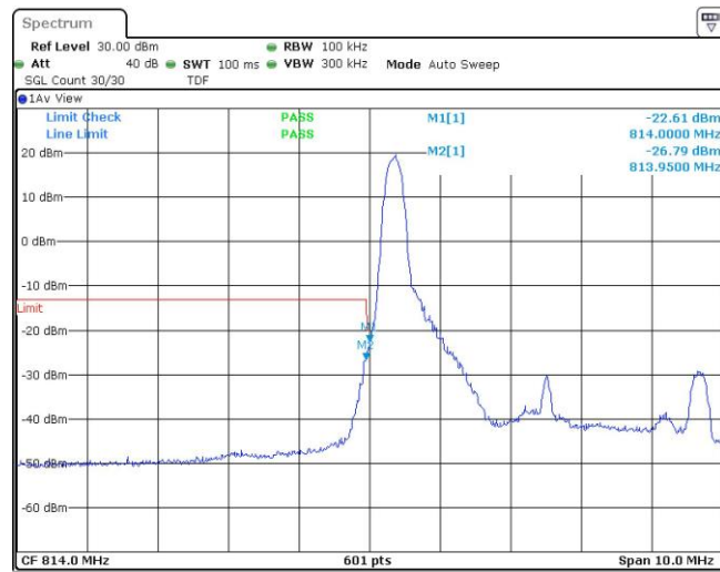
Band26-5MHz-16QAM-26715-1RB#24
