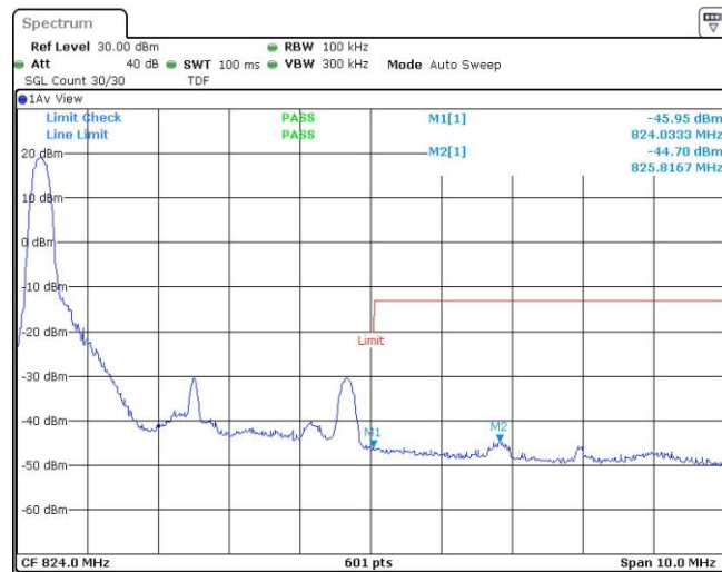
Band26-5MHz-16QAM-26765-1RB#24
