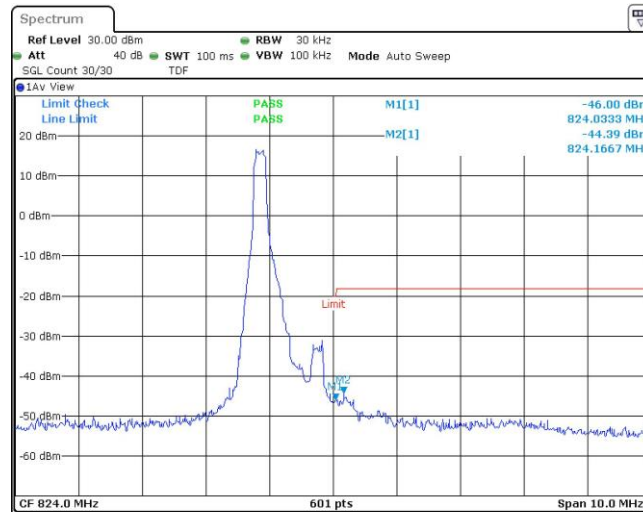
Band26-1.4MHz-QPSK-26783-1RB#5
