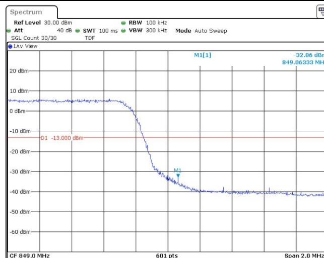
Band26-5MHz-16QAM-26715-1RB#0
