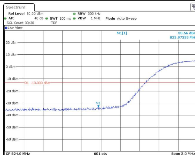
Band26-15MHz-QPSK-26965-1RB#0
