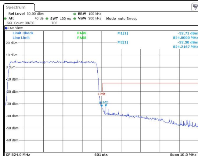
Band26-5MHz-16QAM-26815-1RB#0
