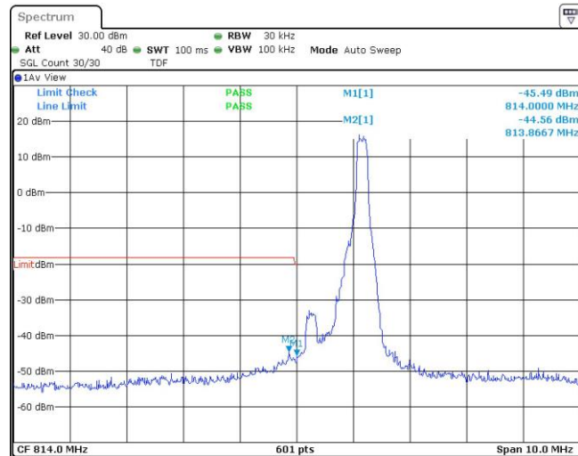
Band26-1.4MHz-16QAM-26697-6RB#0
