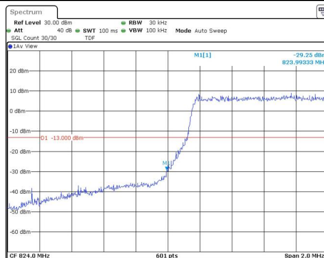
Band26-1.4MHz-16QAM-27033-1RB#0
