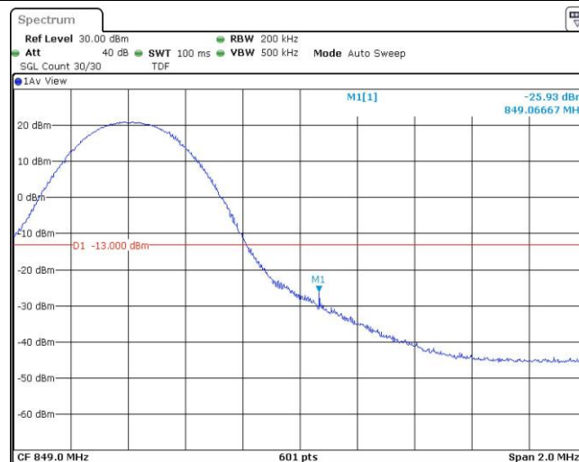
Band26-10MHz-QPSK-26990-50RB#0
