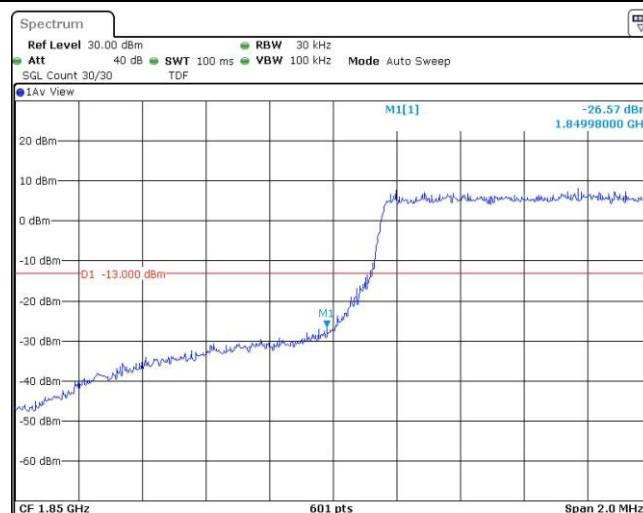
Band25-1.4MHz-16QAM-26683-1RB#0
