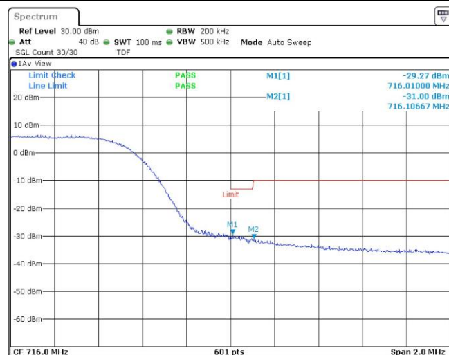
Band17-10MHz-16QAM-23780-1RB#0
