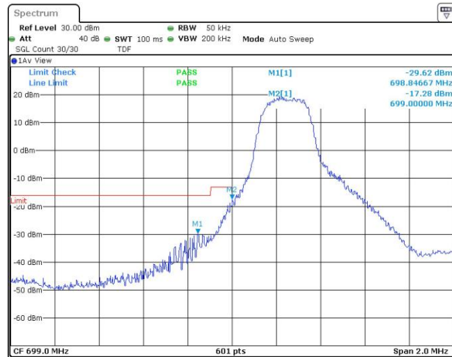
Band12-3MHz-16QAM-23025-1RB#14
