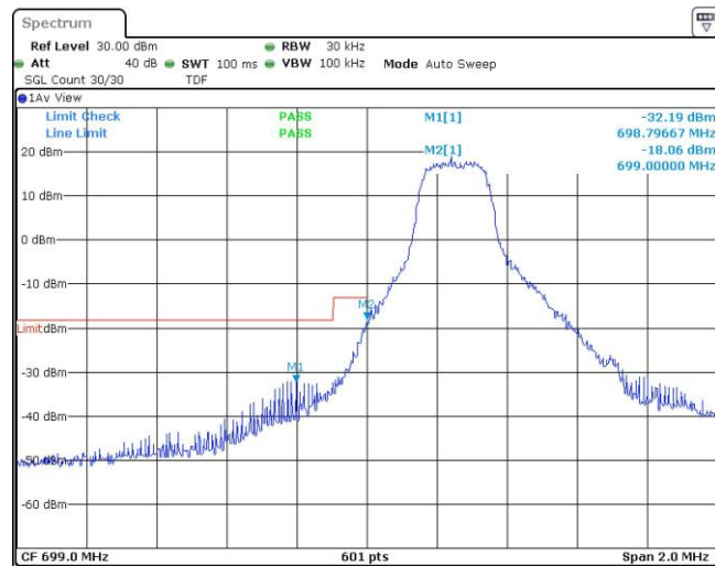
Band12-1.4MHz-QPSK-23017-1RB#5
