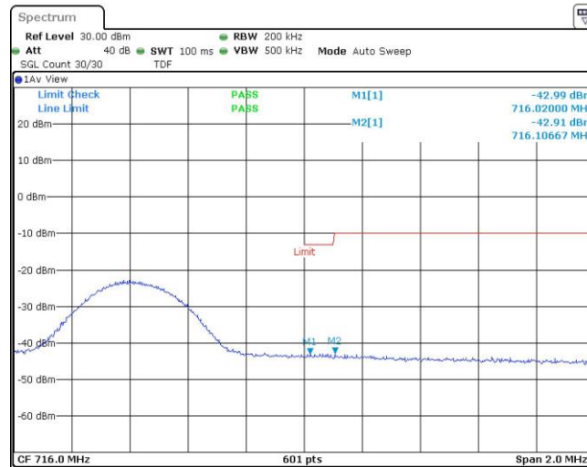
Band17-10MHz-16QAM-23800-1RB#49
