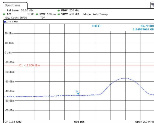
Band25-10MHz-16QAM-26090-50RB#0
