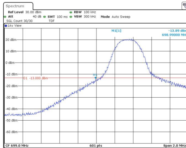
Band12-5MHz-16QAM-23035-1RB#24
