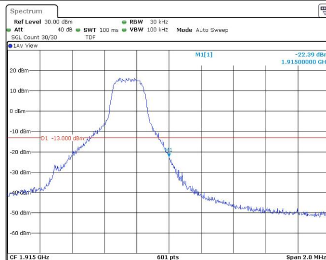
Band25-1.4MHz-QPSK-26683-6RB#0
