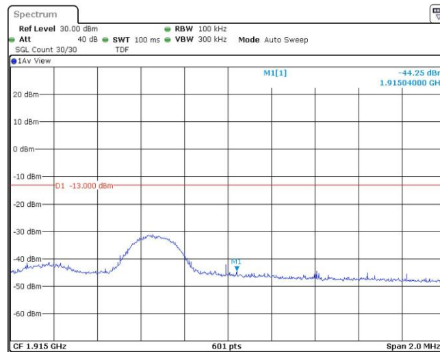
Band25-5MHz-16QAM-26665-1RB#24
