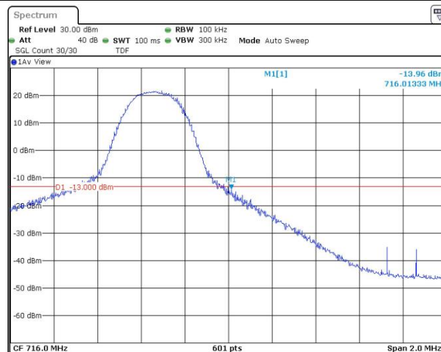
Band17-5MHz-QPSK-23825-25RB#0
