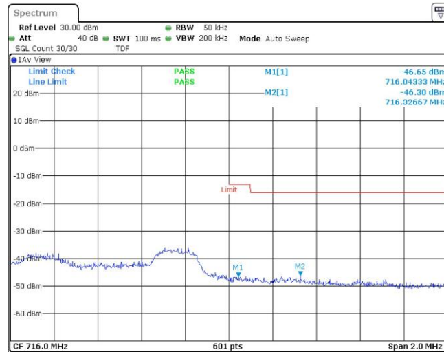
Band12-3MHz-16QAM-23165-1RB#14
