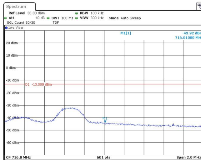
Band17-5MHz-QPSK-23825-1RB#24
