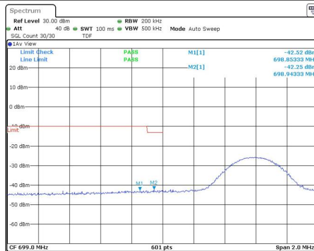
Band12-10MHz-QPSK-23060-50RB#0
