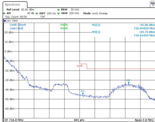
Band12-1.4MHz-16QAM-23173-1RB#5
