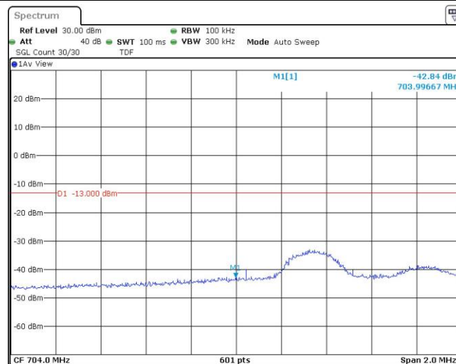
Band17-5MHz-16QAM-23755-25RB#0
