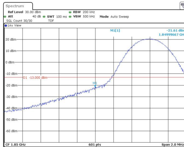
Band25-10MHz-QPSK-26090-1RB#49
