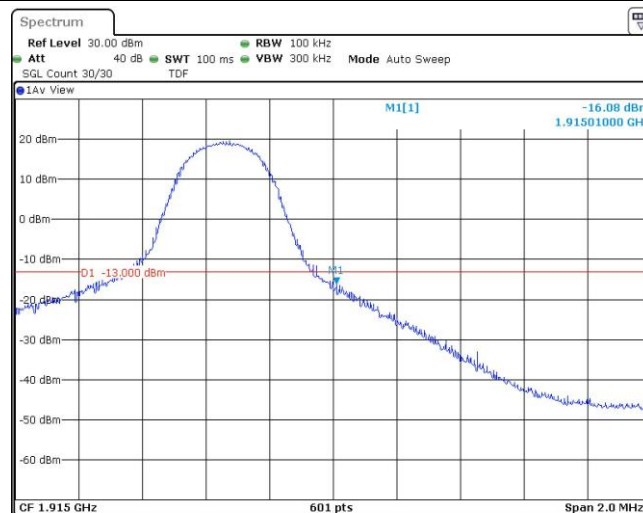
Band25-5MHz-QPSK-26665-25RB#0
