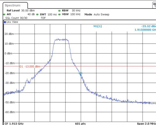
Band25-1.4MHz-16QAM-26683-6RB#0
