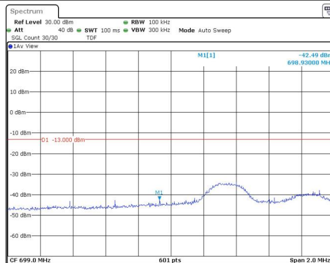
Band12-5MHz-QPSK-23035-25RB#0
