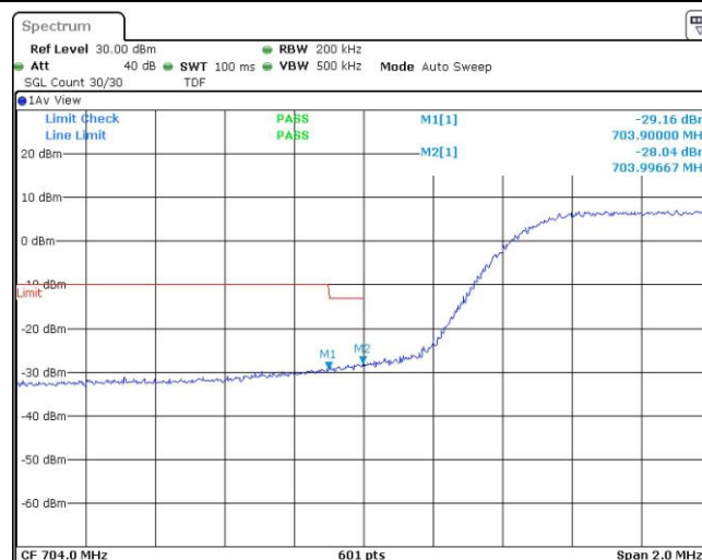
Band17-10MHz-QPSK-23800-1RB#0
