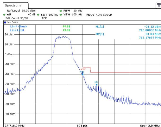
Band12-1.4MHz-QPSK-23173-6RB#0
