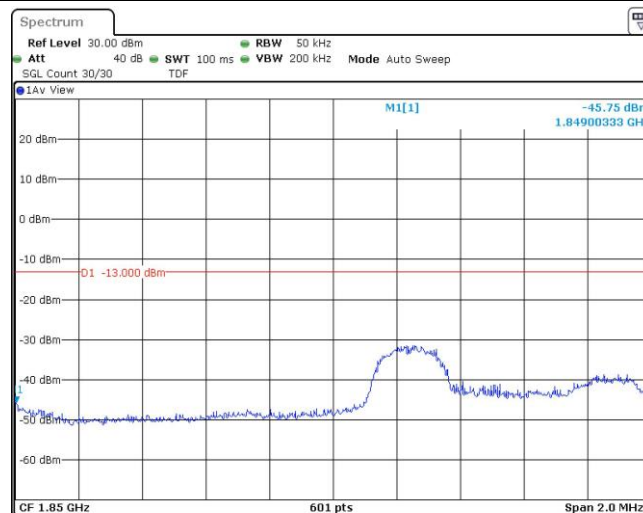
Band25-3MHz-QPSK-26055-15RB#0
