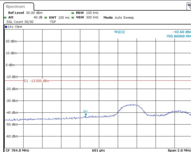
Band17-5MHz-QPSK-23755-25RB#0
