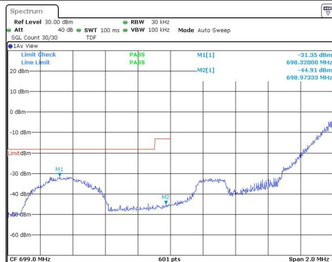
Band12-1.4MHz-QPSK-23017-6RB#0
