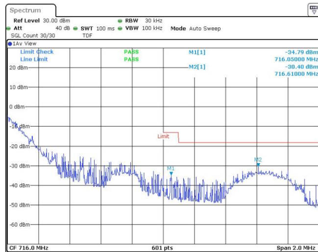
Band12-1.4MHz-QPSK-23173-1RB#5
