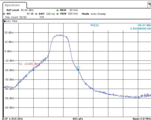
Band25-3MHz-QPSK-26675-15RB#0
