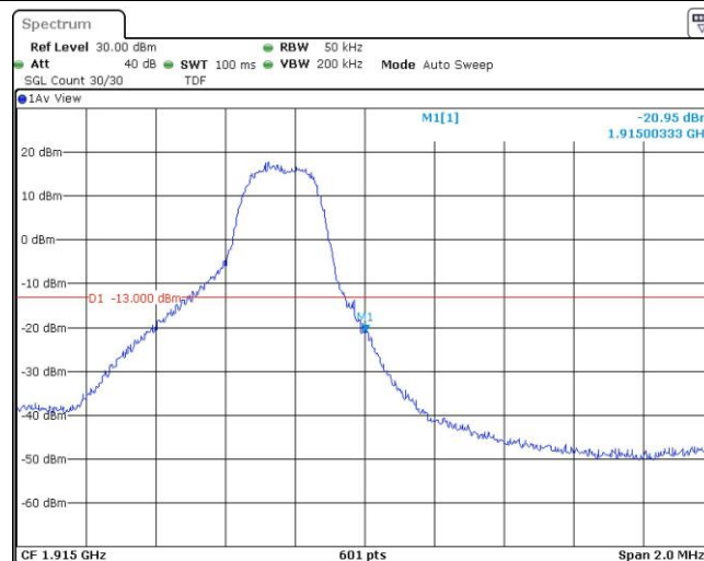
Band25-3MHz-16QAM-26675-15RB#0
