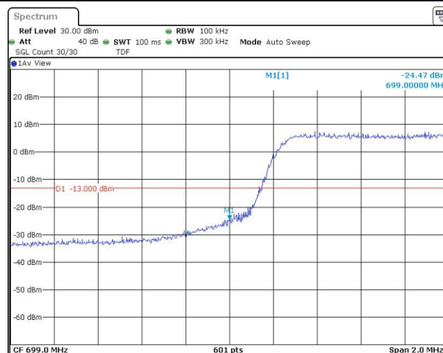
Band12-5MHz-QPSK-23155-1RB#0
