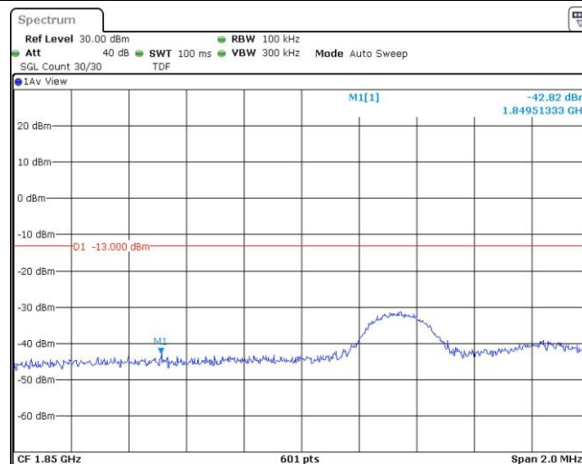
Band25-5MHz-16QAM-26065-25RB#0
