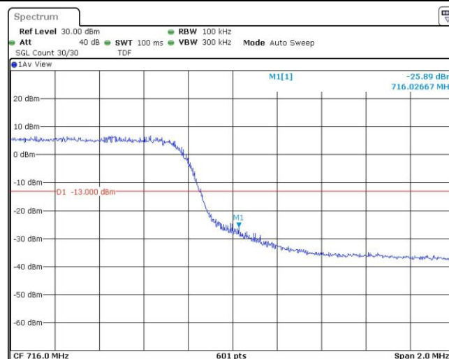
Band17-10MHz-QPSK-23780-1RB#0
