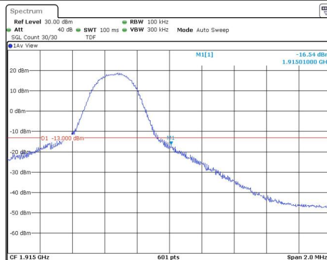
Band25-5MHz-16QAM-26665-25RB#0
