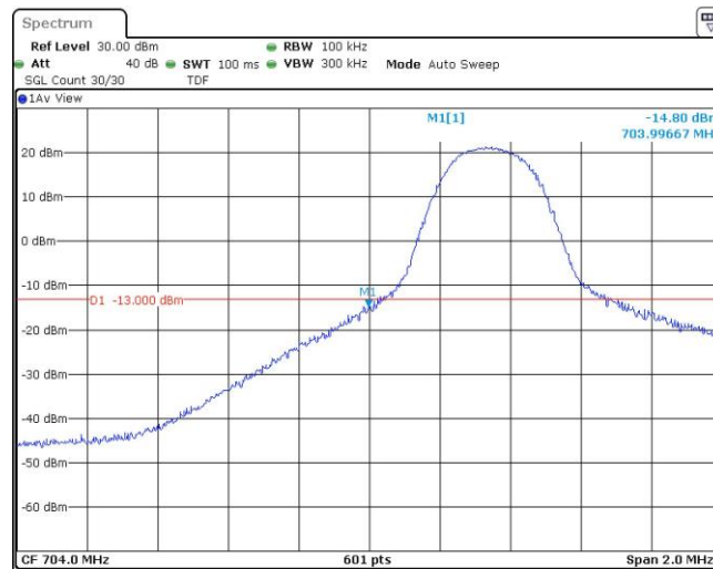
Band17-5MHz-QPSK-23755-1RB#24
