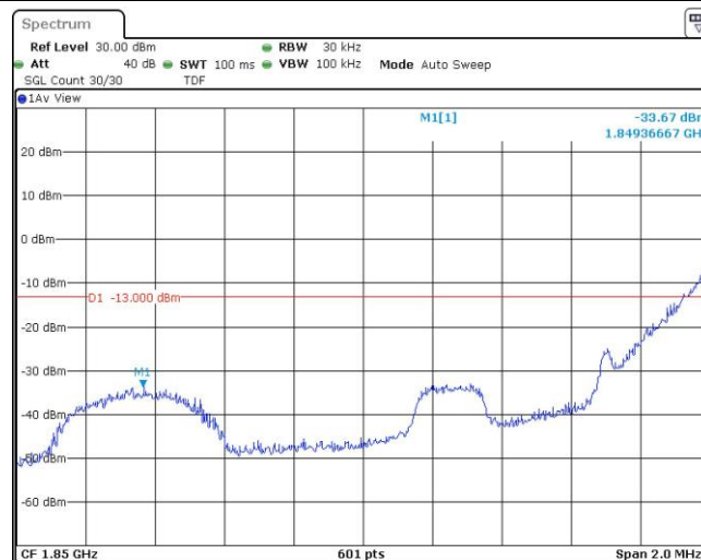
Band25-1.4MHz-16QAM-26047-6RB#0
