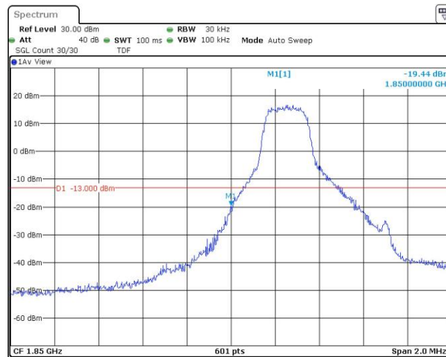
Band25-1.4MHz-QPSK-26047-1RB#5
