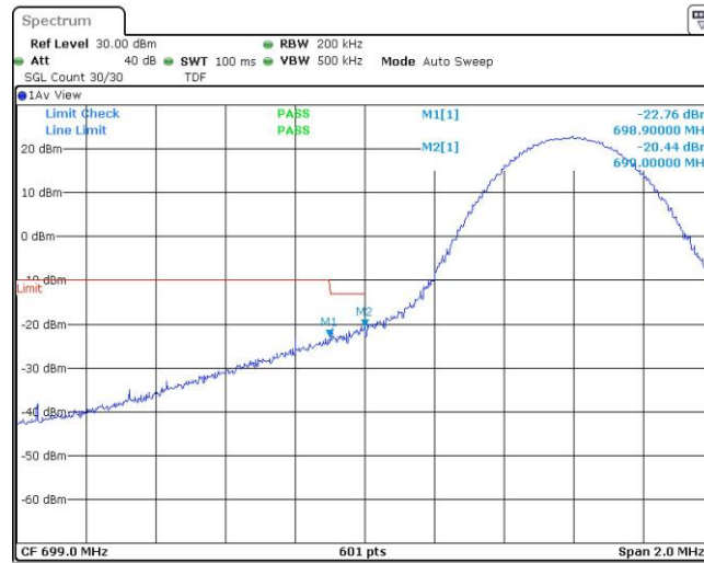
Band12-10MHz-QPSK-23060-1RB#49
