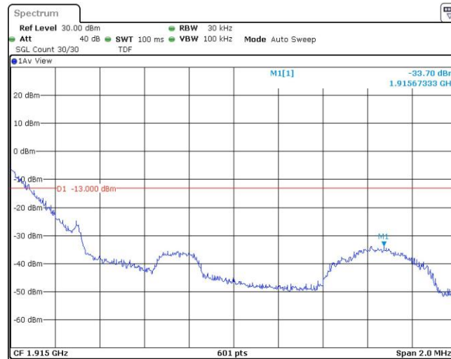
Band25-1.4MHz-QPSK-26683-1RB#5
