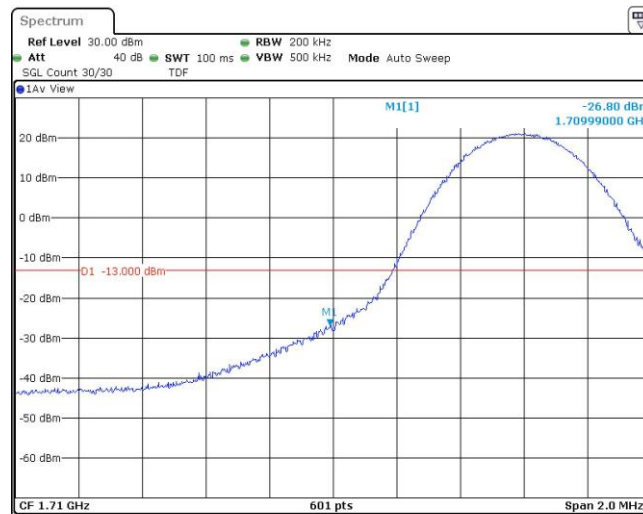
Band4-10MHz-QPSK-20000-1RB#49
