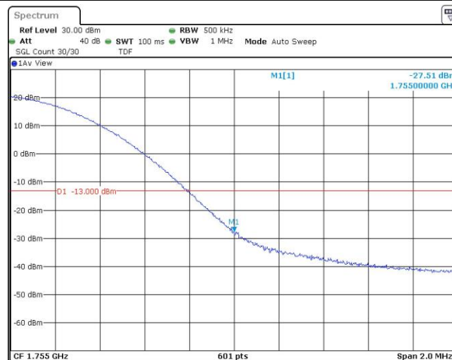
Band4-20MHz-QPSK-20300-100RB#0
