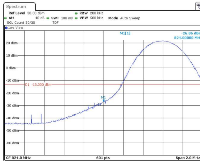
Band5-10MHz-QPSK-20450-1RB#49
