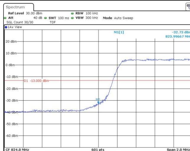
Band5-5MHz-16QAM-20625-1RB#0
