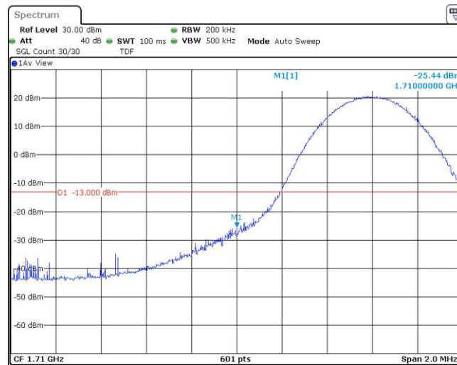
Band4-10MHz-16QAM-20000-1RB#49
