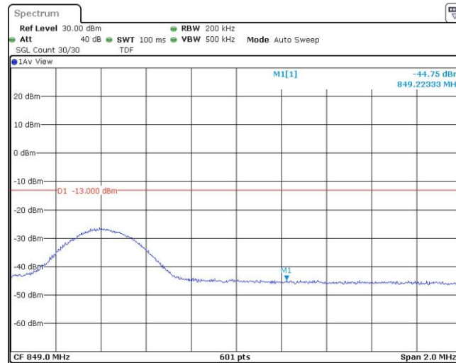
Band5-10MHz-16QAM-20600-1RB#49
