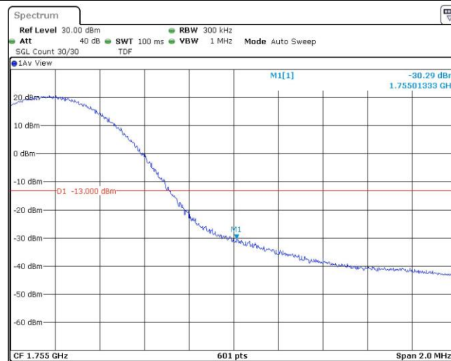
Band4-15MHz-16QAM-20325-75RB#0
