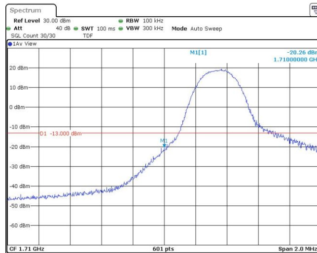
Band4-5MHz-16QAM-19975-1RB#24
