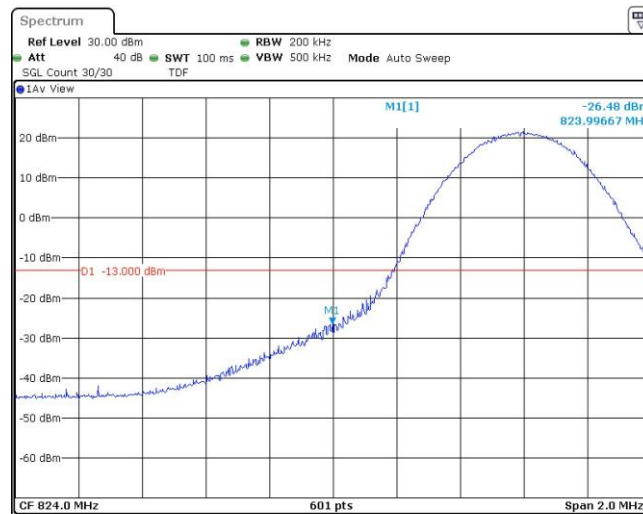
Band5-10MHz-16QAM-20450-1RB#49
