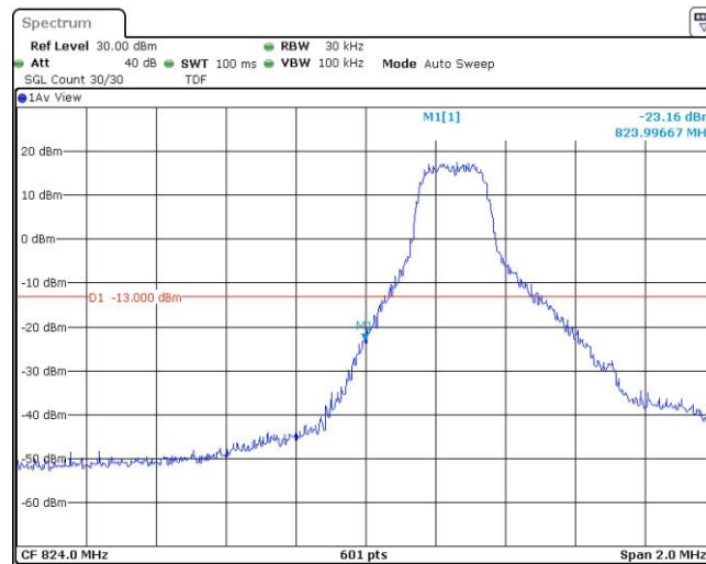
Band5-1.4MHz-QPSK-20407-1RB#5
