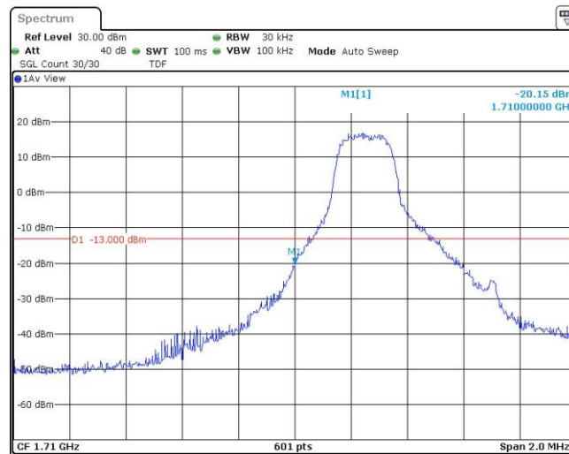
Band4-1.4MHz-QPSK-19957-1RB#5
