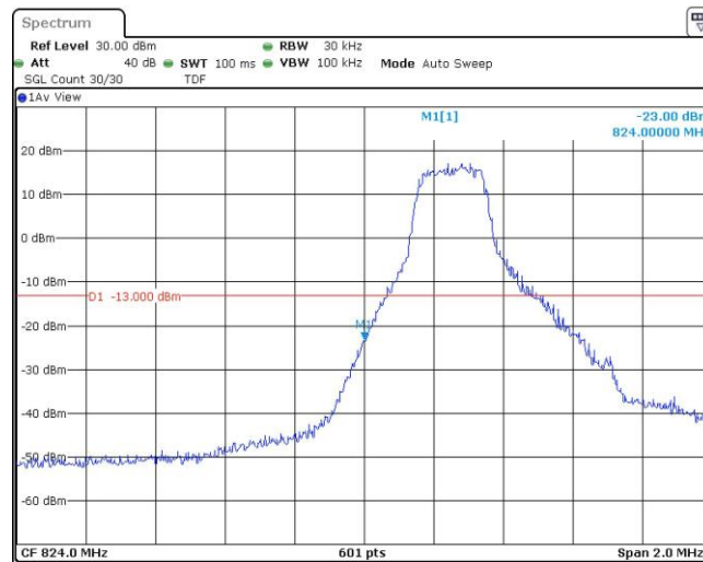
Band5-1.4MHz-16QAM-20407-1RB#5
