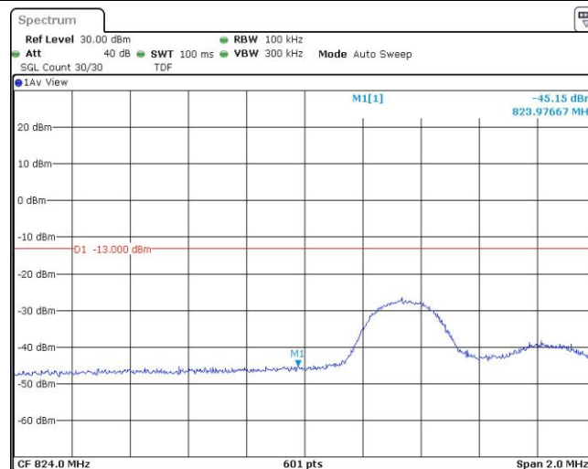
Band5-5MHz-QPSK-20425-25RB#0
