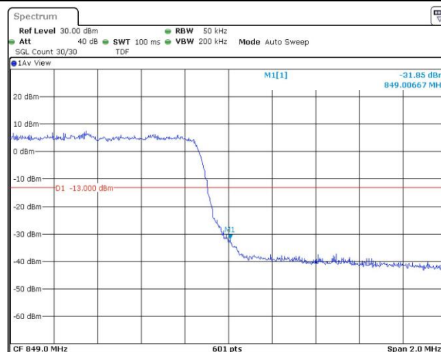
Band5-3MHz-16QAM-20415-1RB#0
