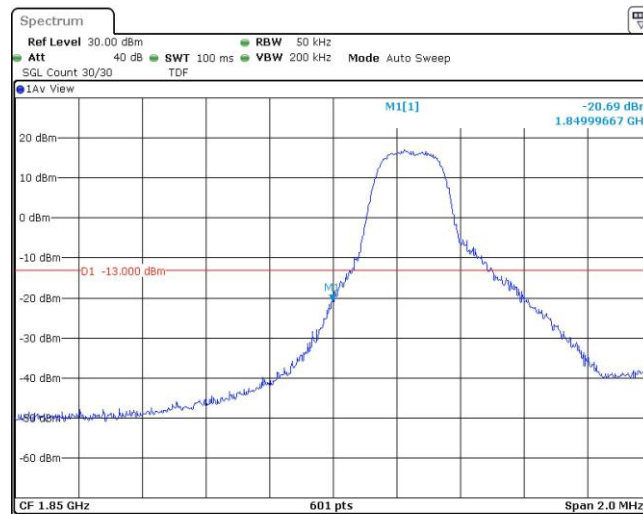
Band2-3MHz-16QAM-18615-1RB#14
