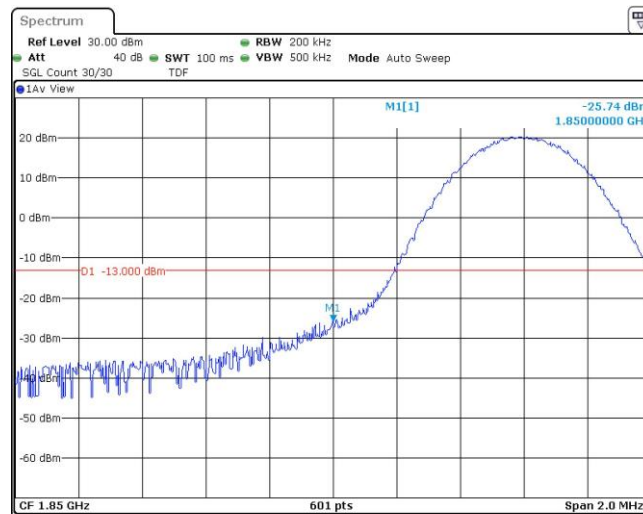
Band2-10MHz-16QAM-18650-1RB#49
