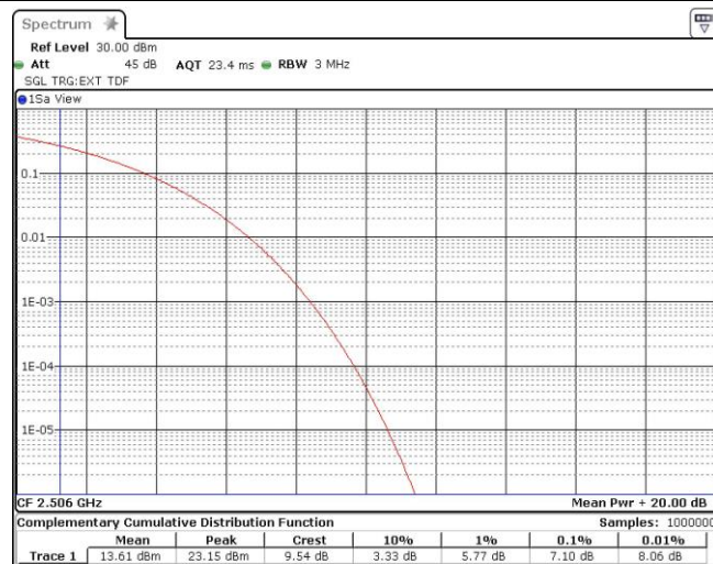
Band41-20MHz-QPSK-40620-1RB#0
