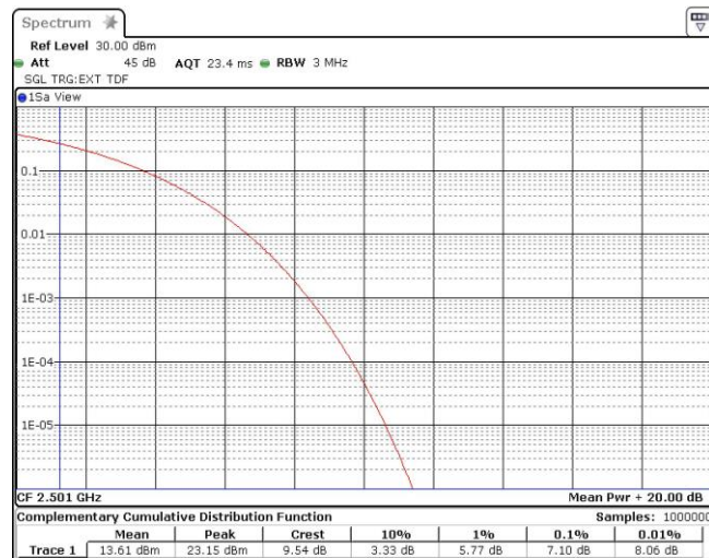
Band41-10MHz-16QAM-39700-50RB#0
