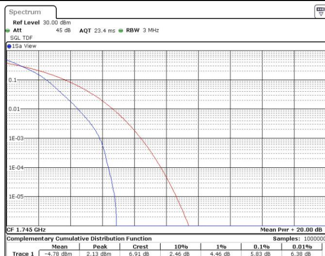
Band66-10MHz-QPSK-132322-1RB#0
