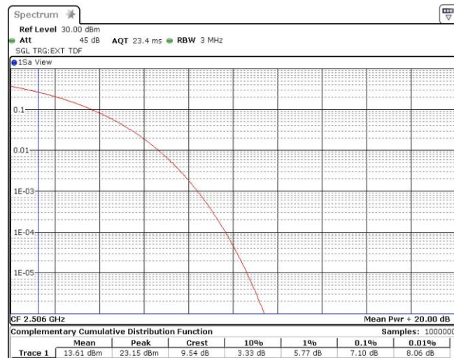
Band41-20MHz-16QAM-39750-100RB#0
