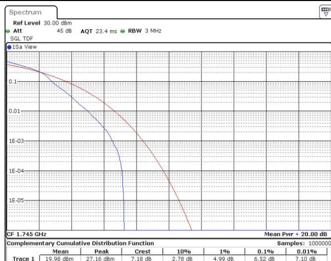
Band66-1.4MHz-16QAM-132322-1RB#0
