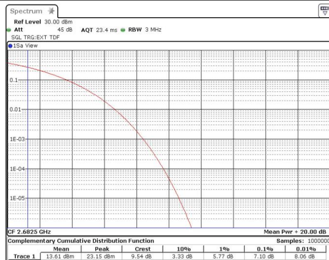
Band41-15MHz-16QAM-41515-75RB#0
