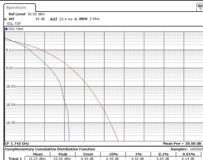
Band66-3MHz-QPSK-132322-1RB#0
