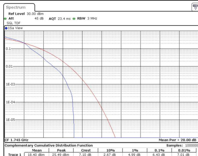
Band66-3MHz-16QAM-132322-1RB#0
