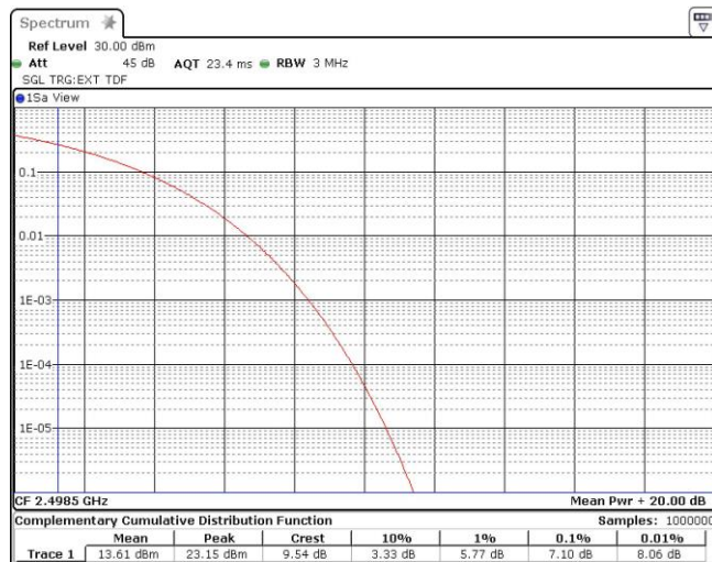
Band41-5MHz-16QAM-39675-25RB#0
