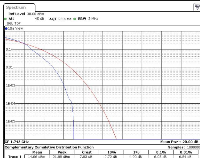
Band66-5MHz-16QAM-132322-1RB#0
