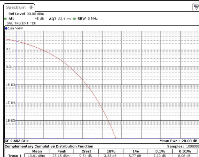
Band41-10MHz-QPSK-41540-50RB#0
