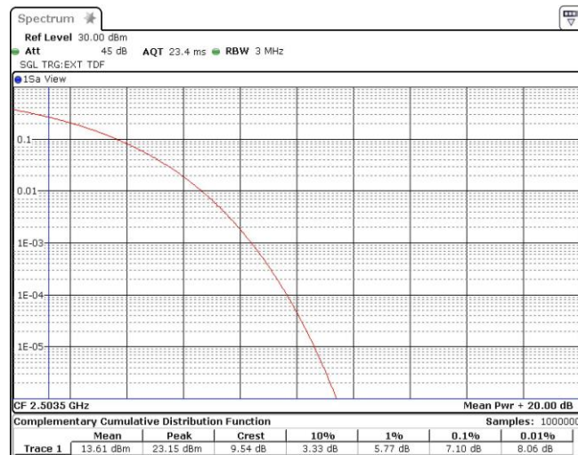
Band41-15MHz-16QAM-39725-75RB#0
