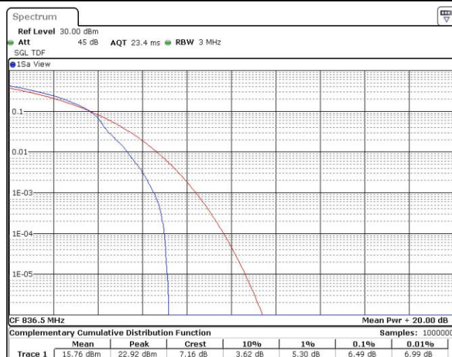
Band26-10MHz-16QAM-26915-50RB#0
