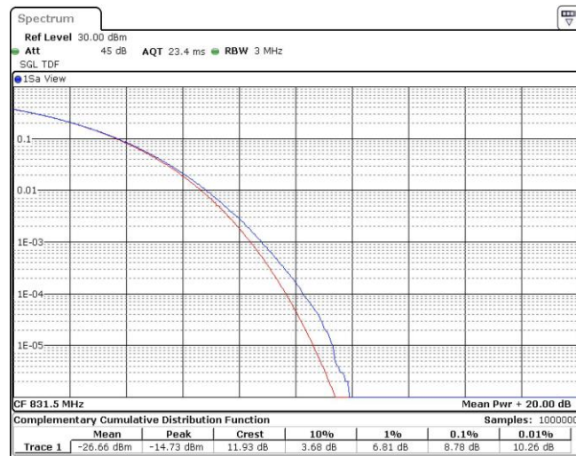
Band26-15MHz-16QAM-26865-75RB#0
