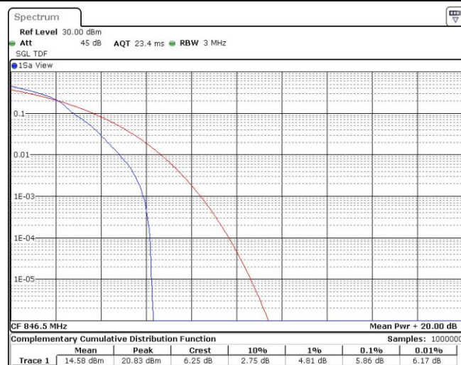
Band26-5MHz-16QAM-27015-25RB#0
