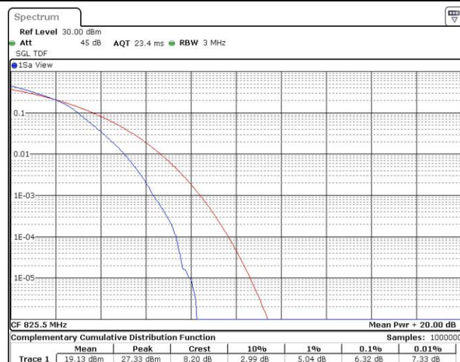
Band26-3MHz-16QAM-26805-15RB#0
