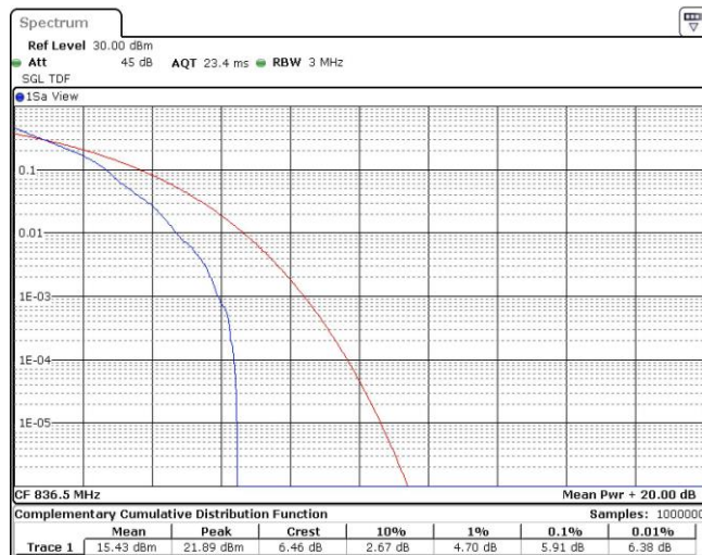
Band26-5MHz-QPSK-26915-25RB#0
