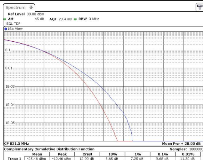
Band26-15MHz-QPSK-26765-1RB#0
