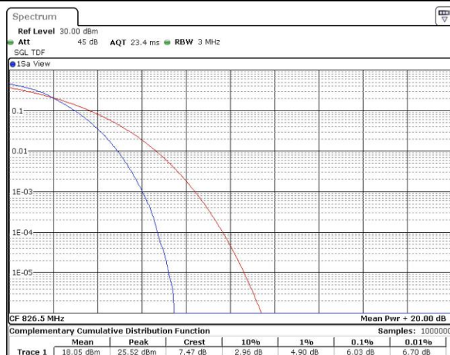
Band26-5MHz-16QAM-26815-25RB#0
