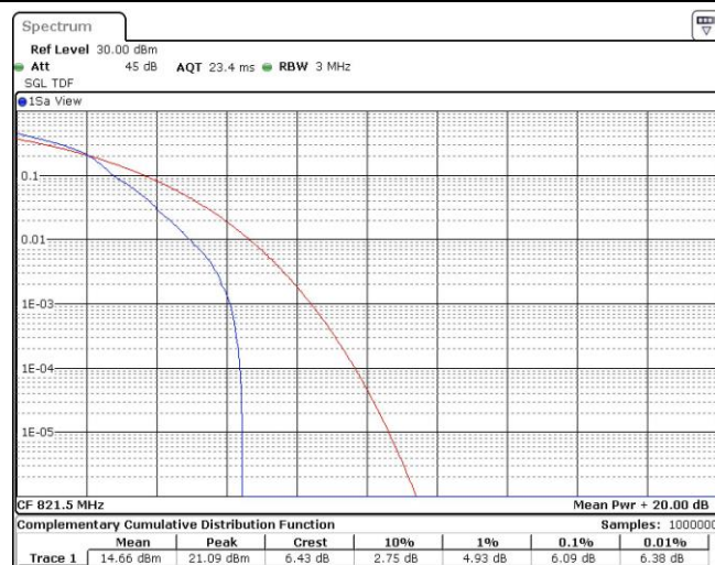
Band26-5MHz-16QAM-26765-25RB#0
