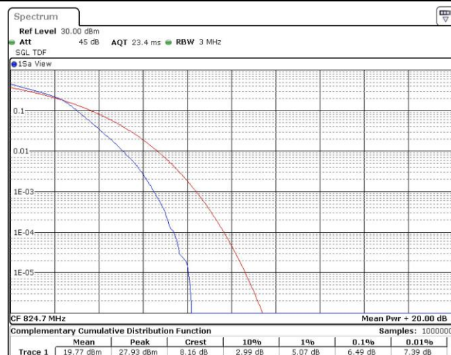
Band26-1.4MHz-16QAM-26797-6RB#0
