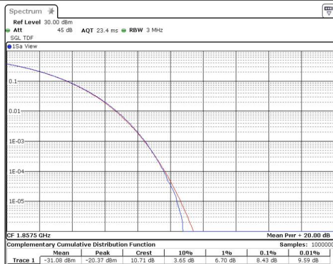
Band25-15MHz-QPSK-26115-75RB#0
