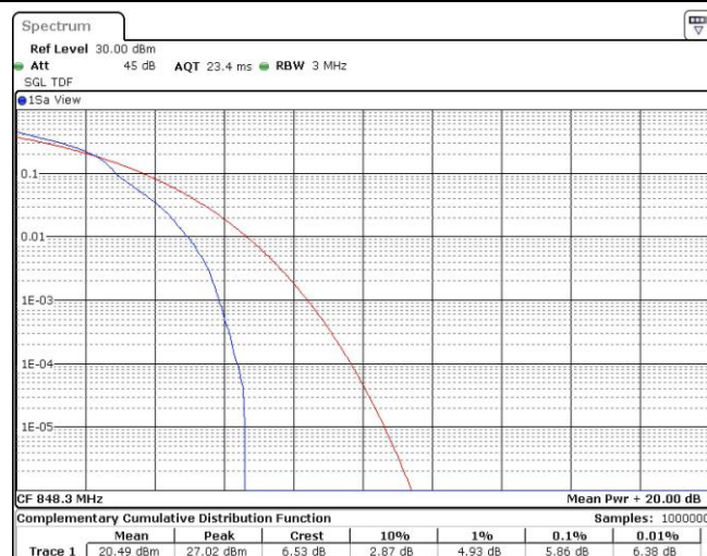
Band26-1.4MHz-16QAM-27033-1RB#0
