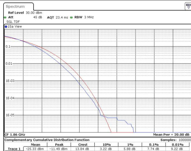
Band25-20MHz-16QAM-26140-100RB#0
