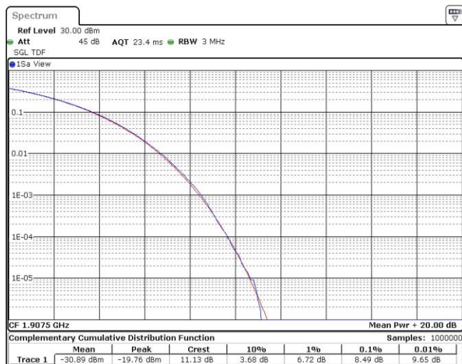
Band25-15MHz-QPSK-26615-75RB#0
