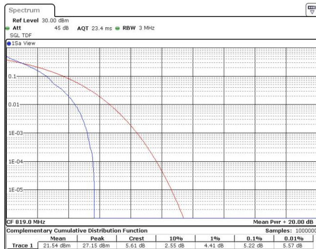
Band26-1.4MHz-QPSK-26740-6RB#0
