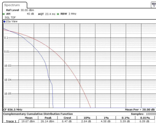
Band26-3MHz-QPSK-26915-15RB#0
