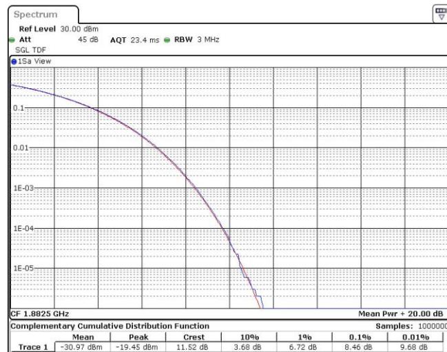
Band25-15MHz-16QAM-26365-75RB#0
