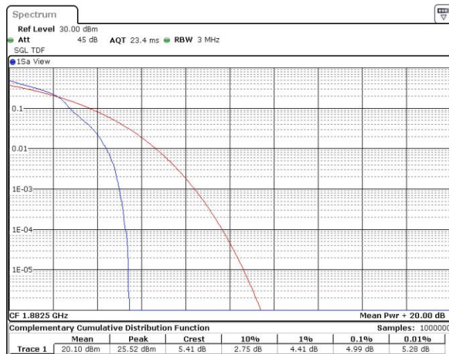
Band25-1.4MHz-16QAM-26365-6RB#0
