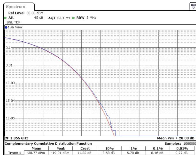
Band25-10MHz-16QAM-26090-50RB#0
