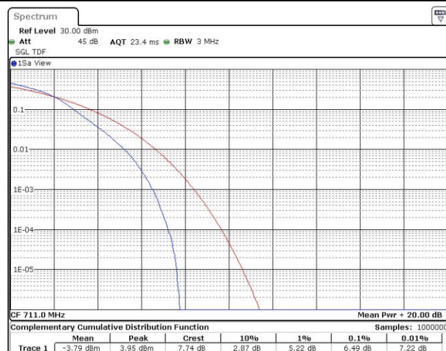
Band17-10MHz-16QAM-23800-1RB#0
