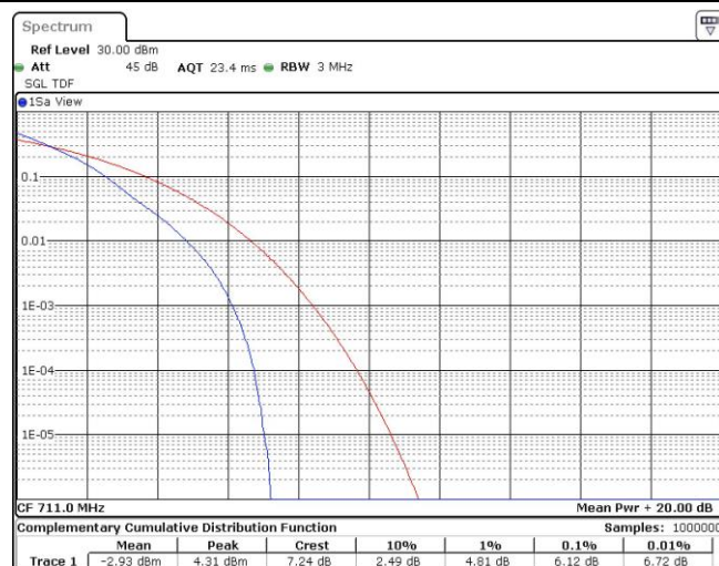
Band17-10MHz-QPSK-23800-1RB#0
