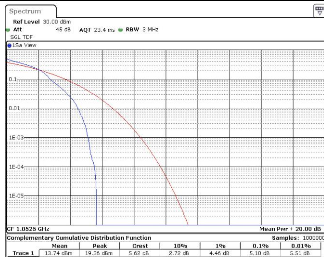
Band25-5MHz-16QAM-26065-25RB#0
