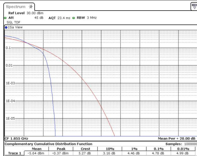
Band25-10MHz-QPSK-26090-50RB#0
