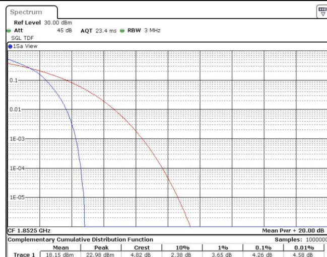
Band25-5MHz-QPSK-26065-25RB#0
