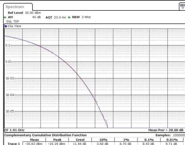
Band25-10MHz-16QAM-26640-1RB#0
