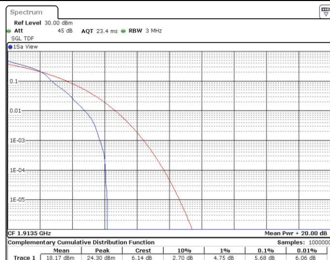
Band25-3MHz-16QAM-26675-1RB#0
