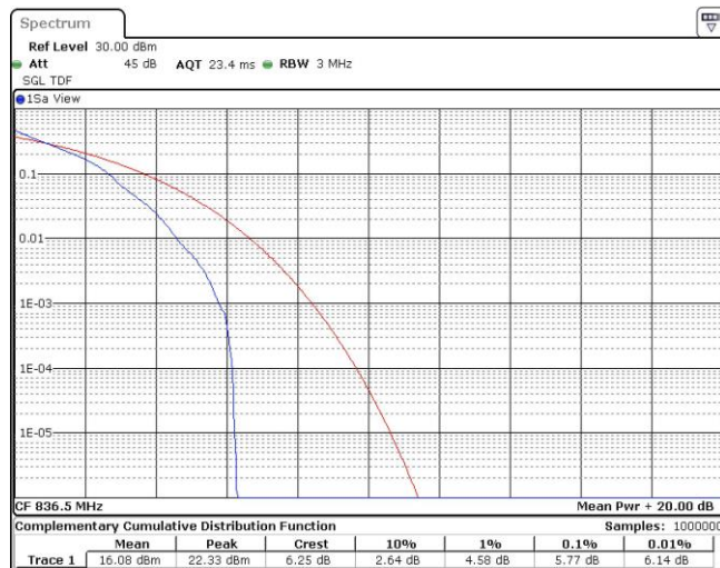
Band5-5MHz-QPSK-20525-25RB#0
