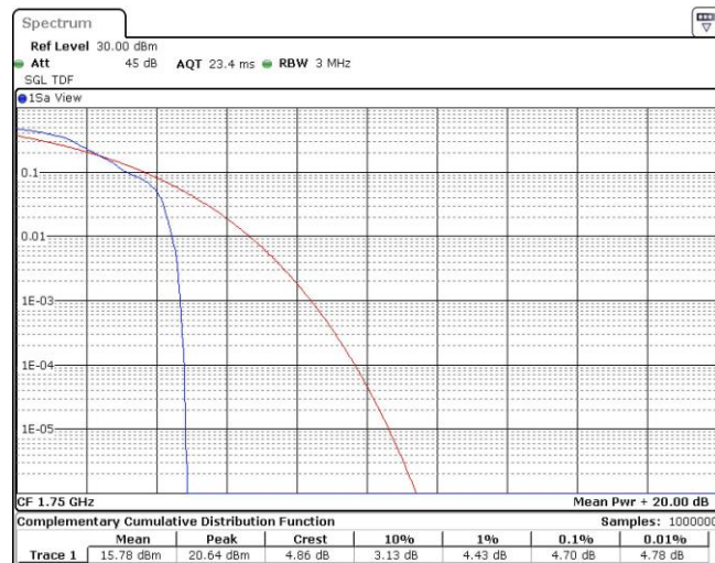
Band4-10MHz-16QAM-20000-1RB#0
