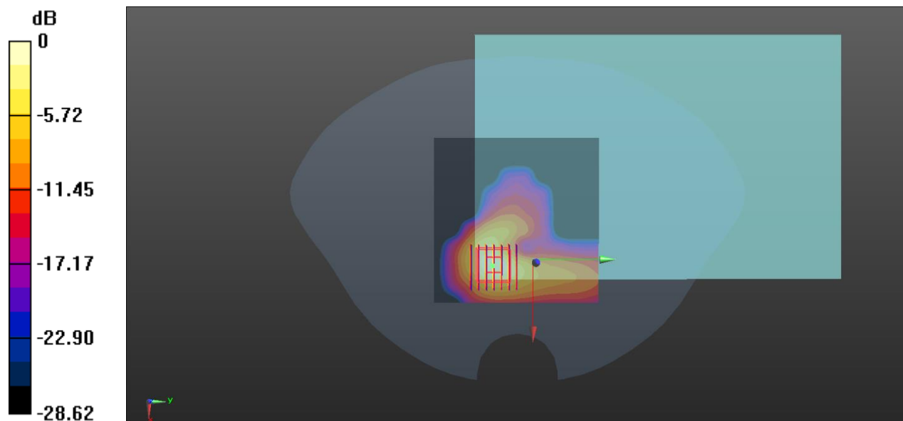
0 dB = 0.705 W/kg
