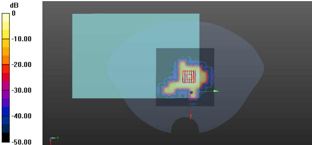
0 dB = 0.328 W/kg
