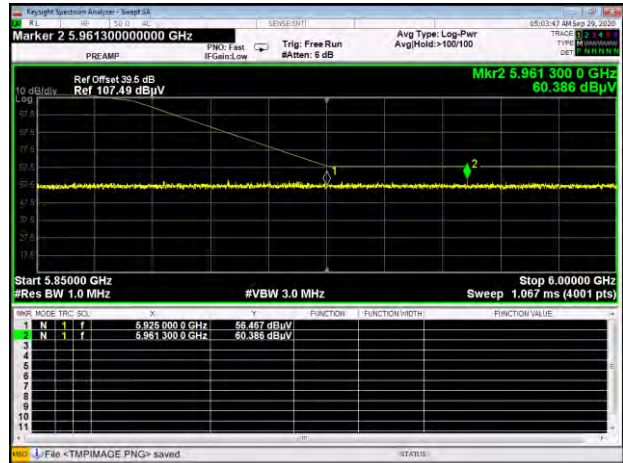
Band 3 11ac20 CH165 Peak
