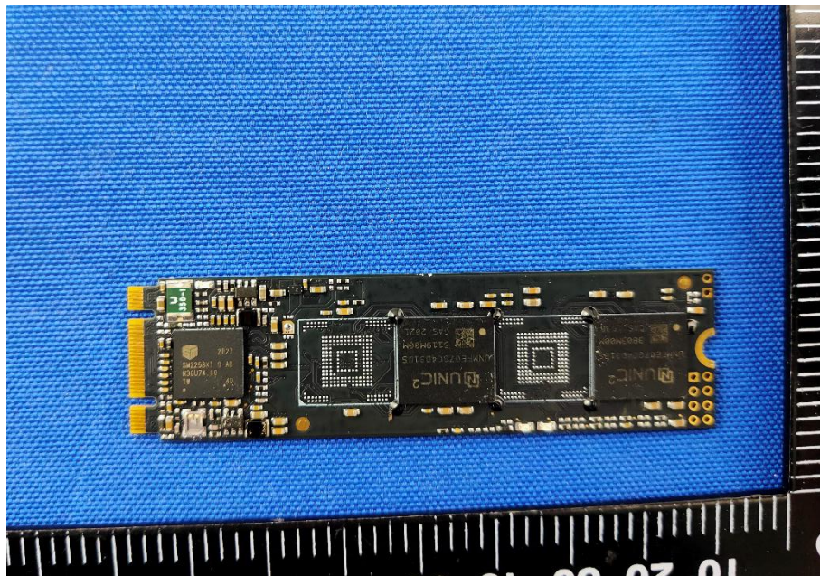
SECONDARY BOARD 2 TOP VIEW (WITHOUT SHIELDING)
