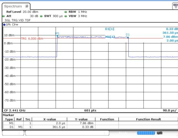
GFSK DH1
