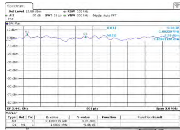
8-DPSK
