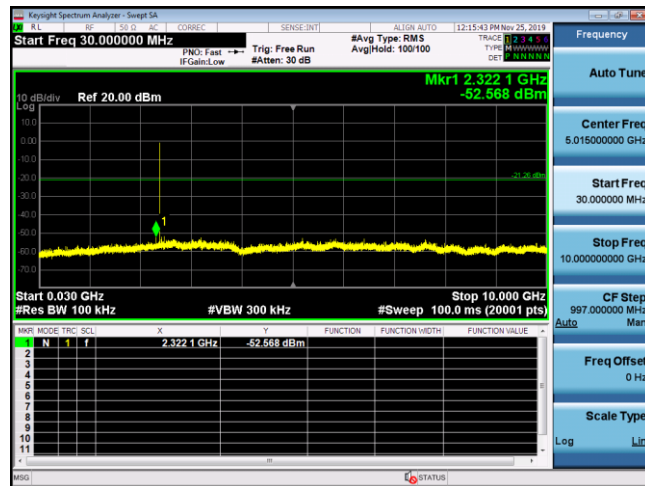
30MHz-10GHz
