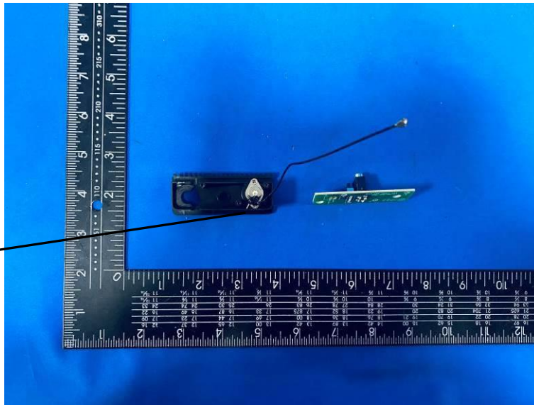
Receiving Antenna
