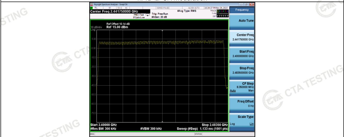
8DPSK Modulation
