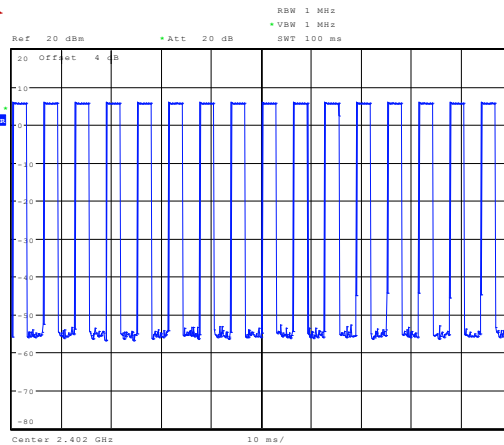
2DH5 on time (Count Pulses) Plot on Channel 00
