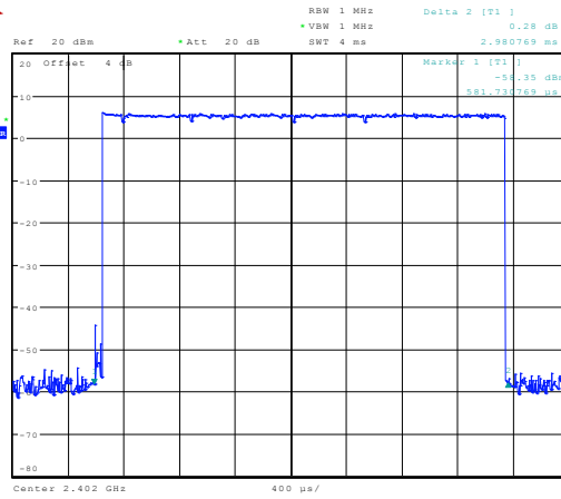
2DH5 on time (One Pulse) Plot on Channel 00
