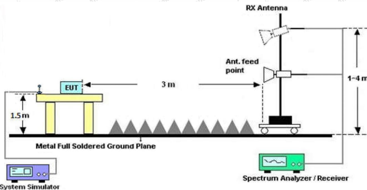
Figure 3. Above 1 GHz
