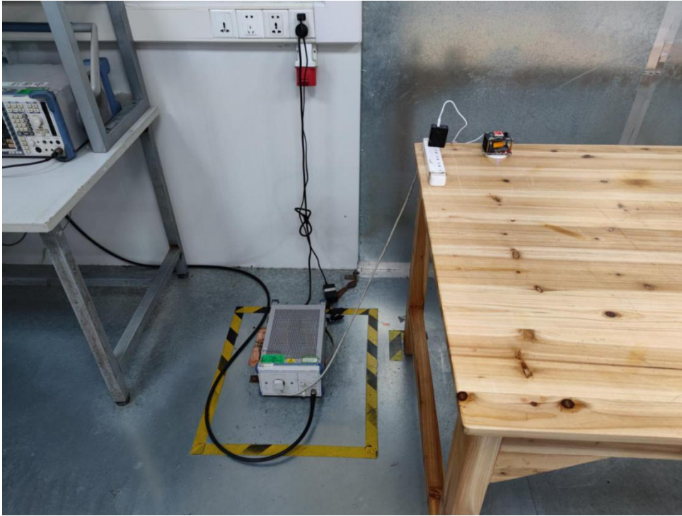
FCC ID: 2APU5-WPC388A Photo of Conducted Emission Measurement
