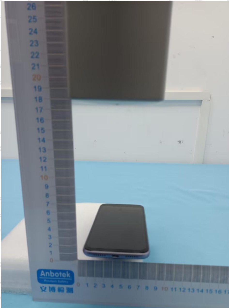
Photo of MPE Measurement at 20 cm
